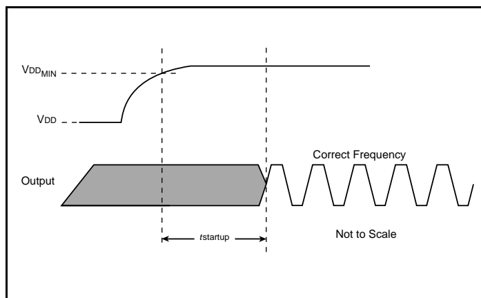
Start-Up Time
