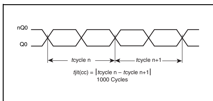
Cycle-to-Cycle Jitter
