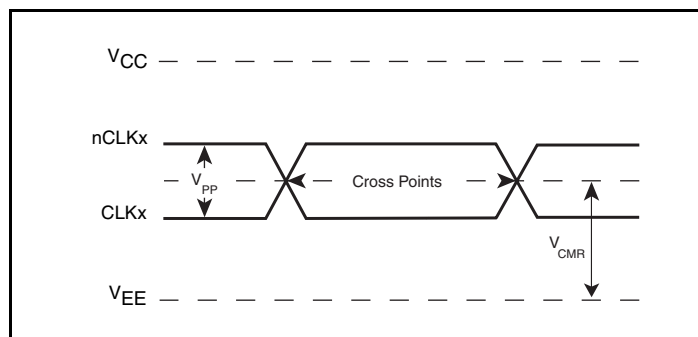
Differential Input Levels
