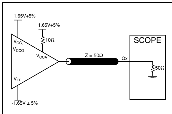
3.3 Core/3.3V LVCMOS Output Load Test Circuit
