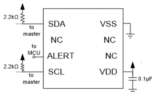
Figure 10. HS40xx Application Circuit – Top View
