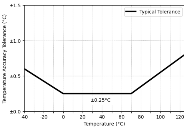
Figure 7. HS40x3 Temperature Sensor Accuracy Tolerance
