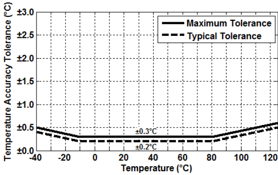
Figure 6. HS3001-ML1 Temperature Sensor Accuracy Tolerance
