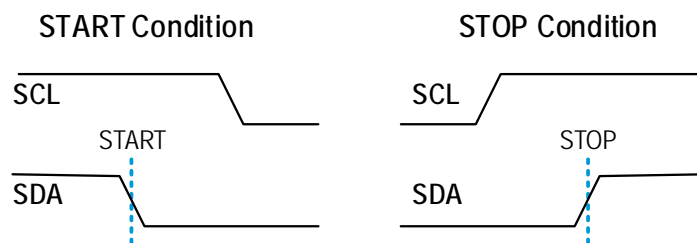
Figure 9. START and STOP Condition Waveform
