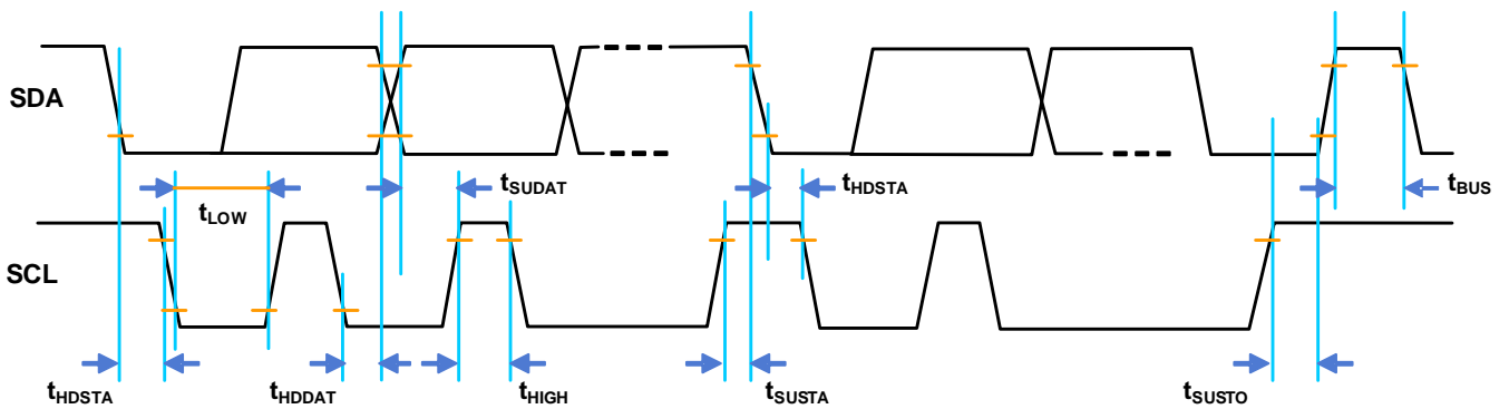
Figure 9. Timing Diagram
