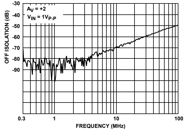
FIGURE 20. OFF ISOLATION
