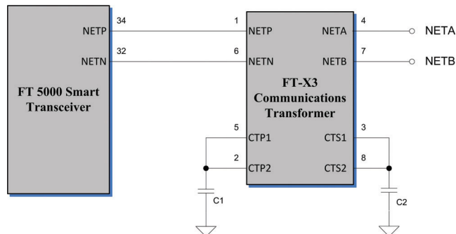
Figure 7. FT-X3 Pin Configuration and Pin-out
