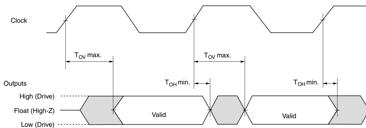
Figure 2-3: Output Delay Waveforms
