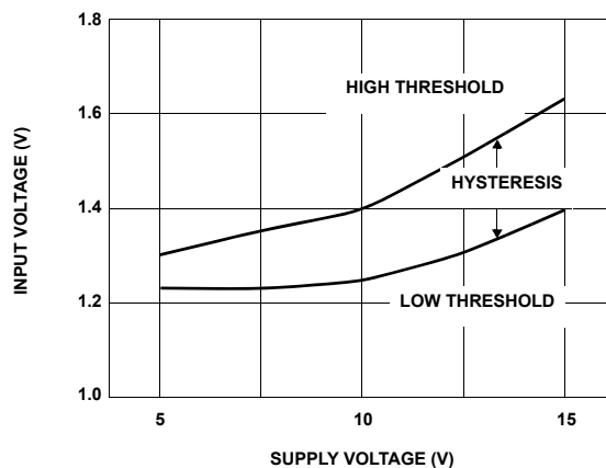
FIGURE 3. INPUT THRESHOLD vs SUPPLY VOLTAGE, T = 25^{\circ}\text{C}
