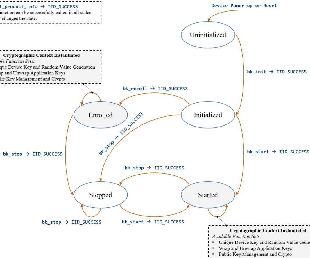
Figure 3 BroadKey state diagram.
