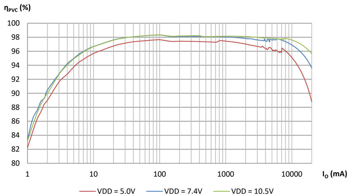
Figure 10: DA9313 Efficiency Automatic Mode Master/Slave
