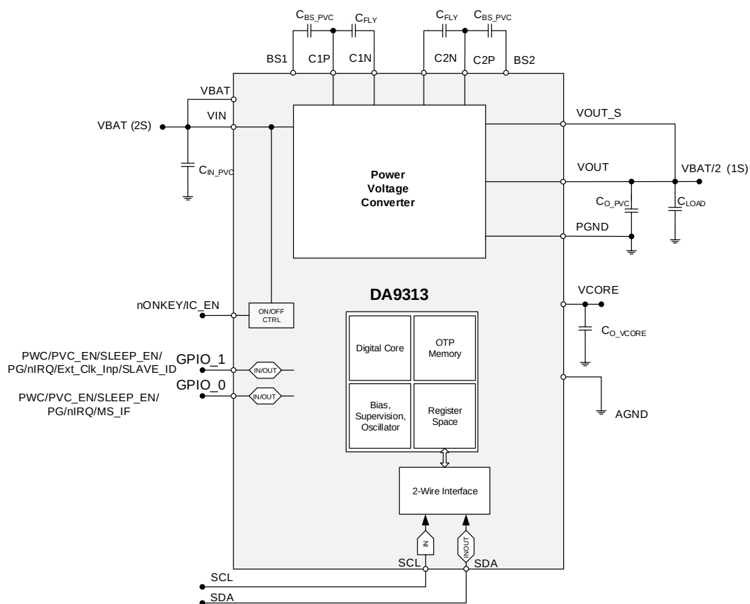
Figure 3: Functional Block Diagram Standalone (I²C Connected)
