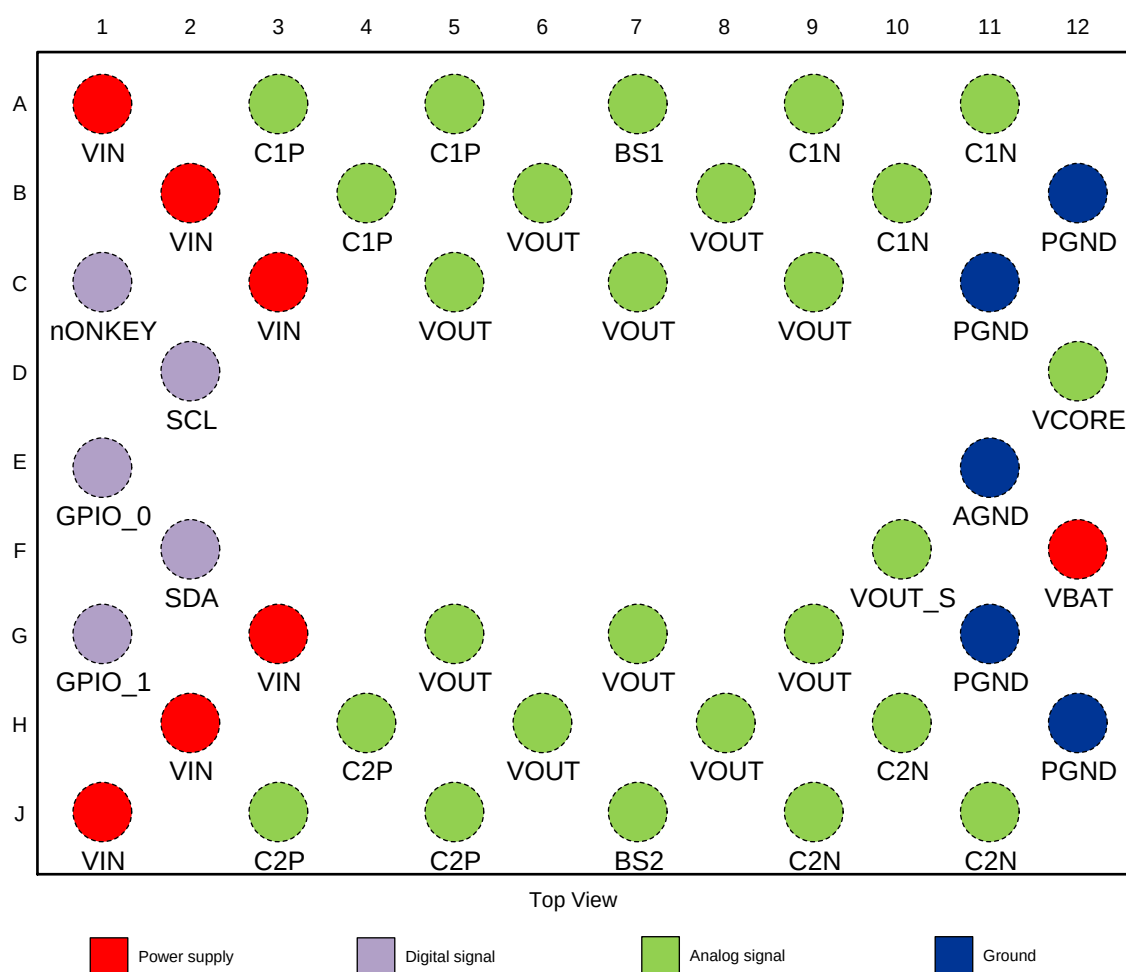
Figure 5: Connection Diagram
