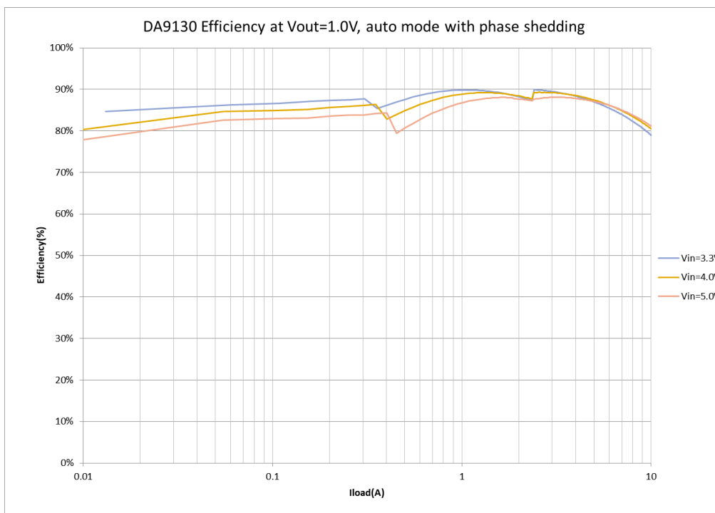
Figure 7. DA9130-A Efficiency, Auto Mode with Phase Shedding
