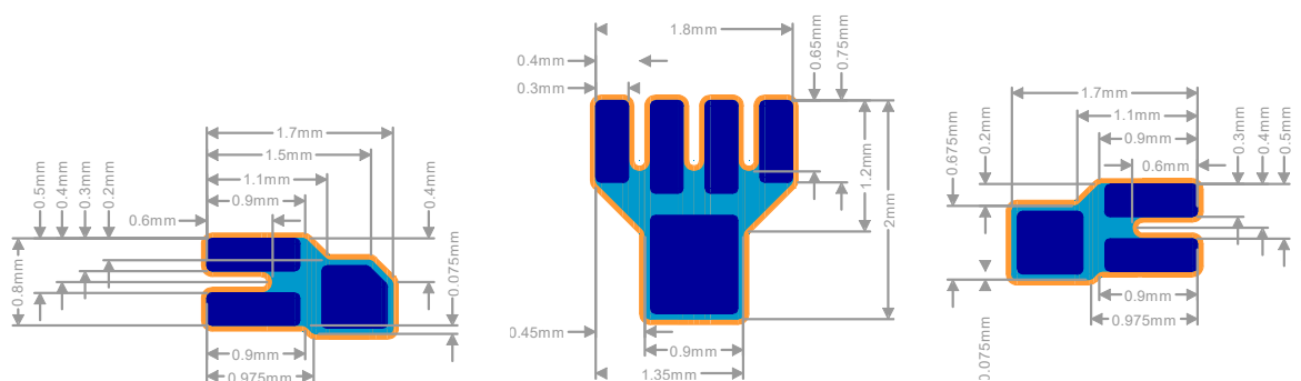
Figure 16. DA9130-A Footprint Details
