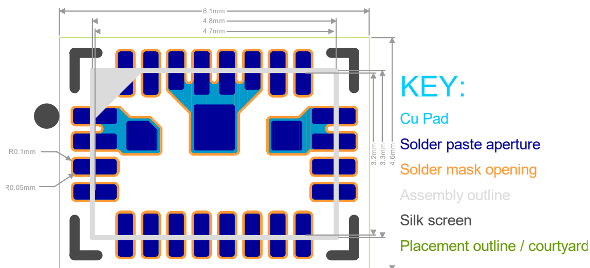
Figure 15. DA9130-A Footprint
