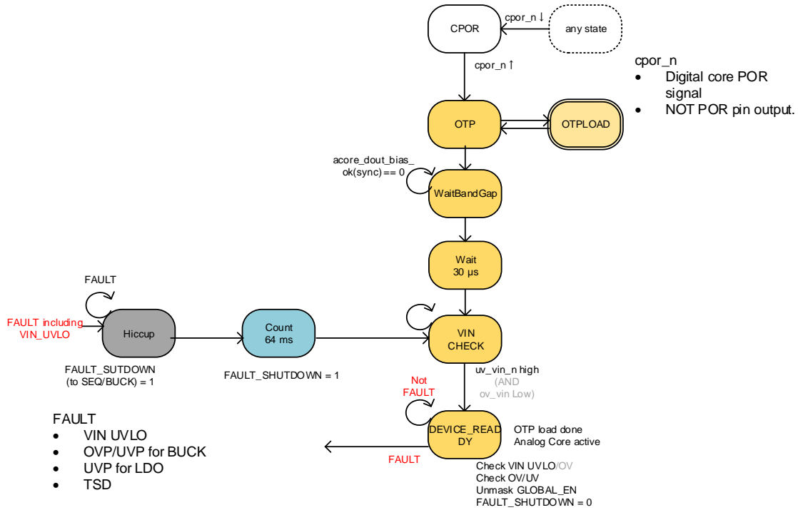
Figure 6: FSM States
