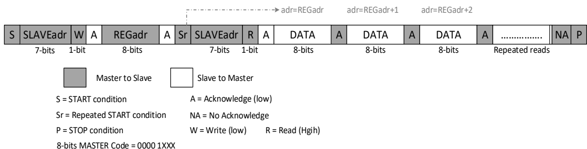
Figure 15: Consecutive Read Command
