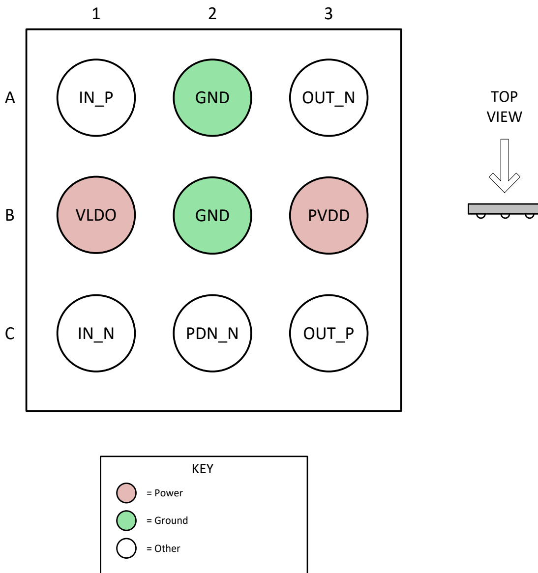
Figure 2: Connection diagram
