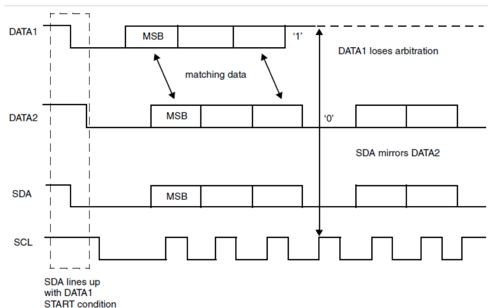
Figure 88: Multiple Master Arbitration
