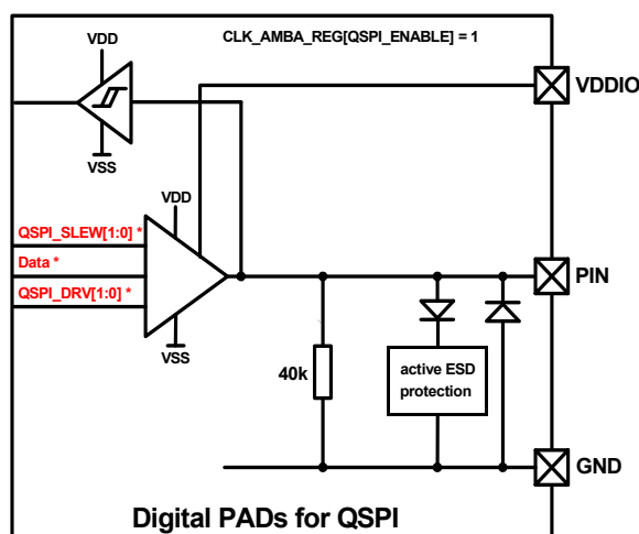
Figure 114: Latching of QSPI pad signals
