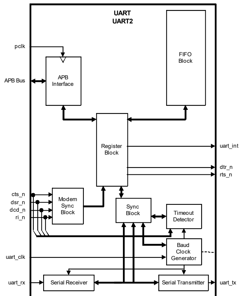
Figure 67: UART Blockdiagram
