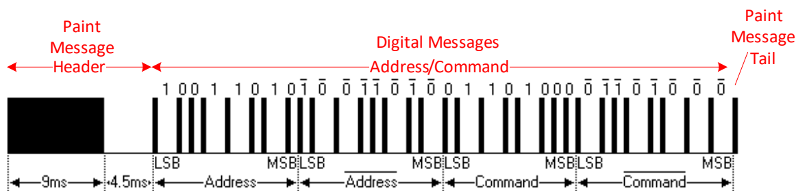
Figure 91: Paint/Digital messages on a NEC based example
