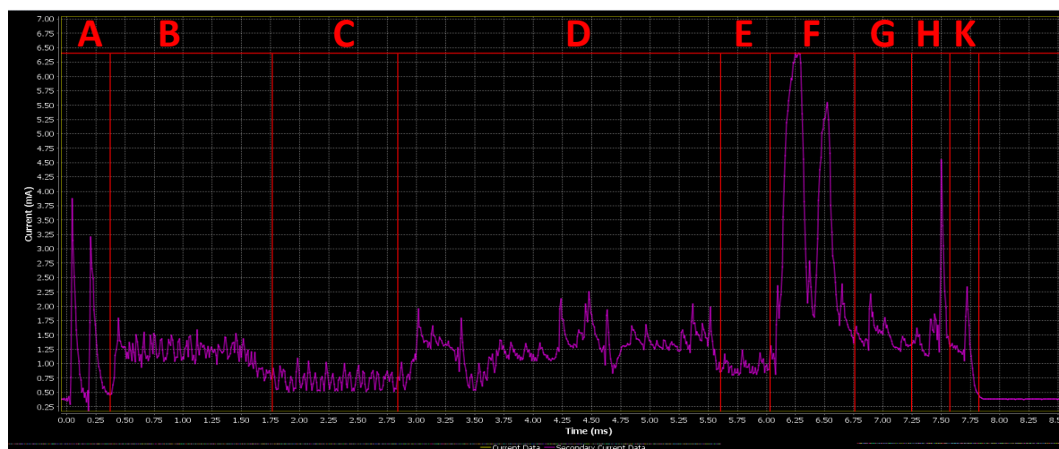
Figure 123: BLE Connection power profile
