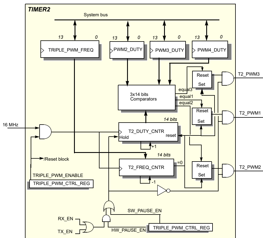
Figure 101: PWM Timer 2 block diagram
