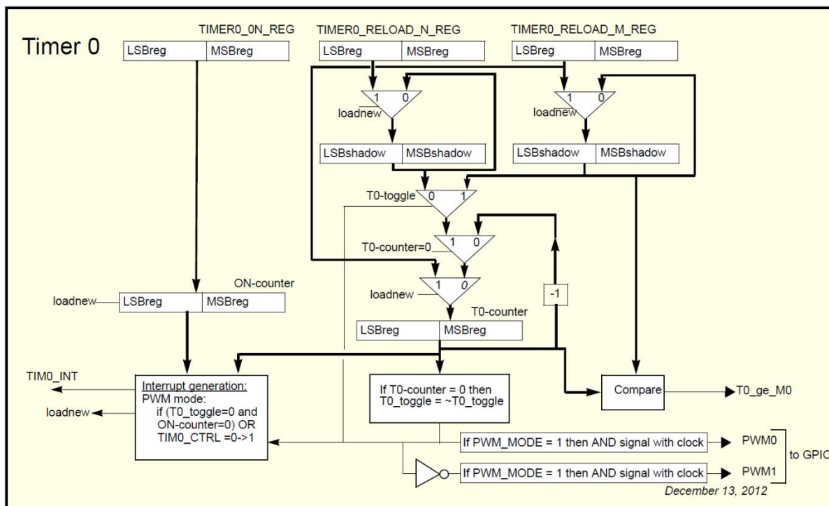
Figure 50. Timer 0 block diagram
