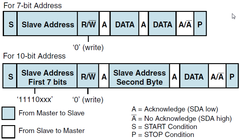
Figure 31. Master-transmitter protocol
