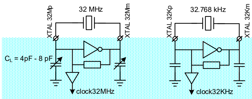
Figure 19. Crystal oscillator circuits
