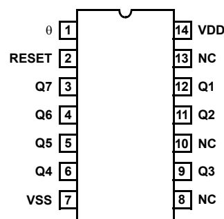
CD4024BMS TOP VIEW
