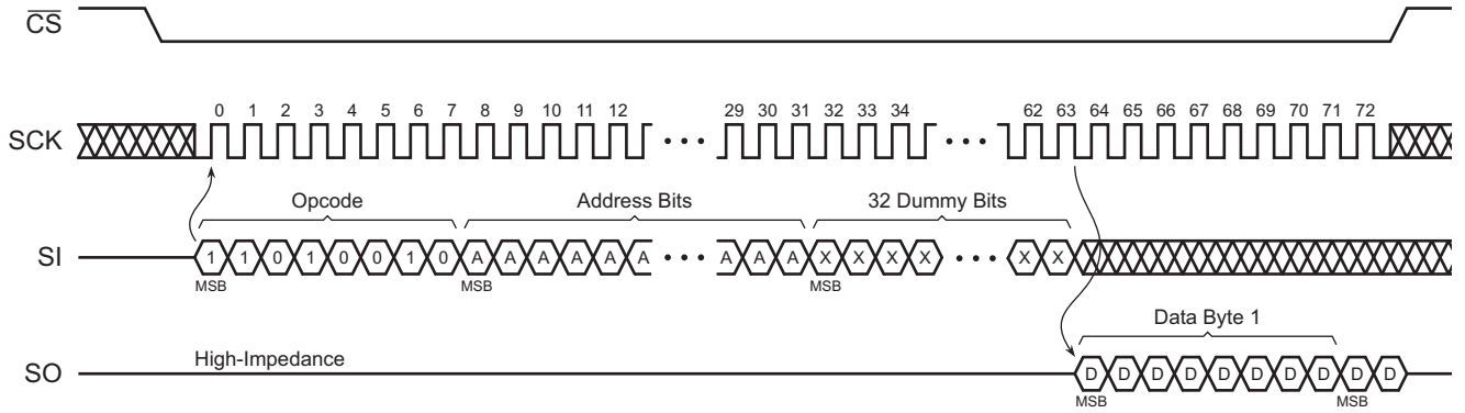
Figure 44. Main Memory Page Read Timing (Opcode D2h)
