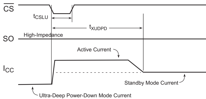
Figure 19. Exit Ultra-Deep Power-Down
