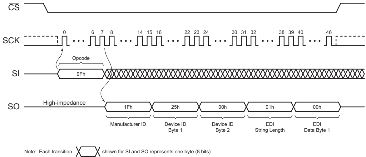
Figure 51. Manufacturer and Device Read Timing (Opcode 9Fh)
