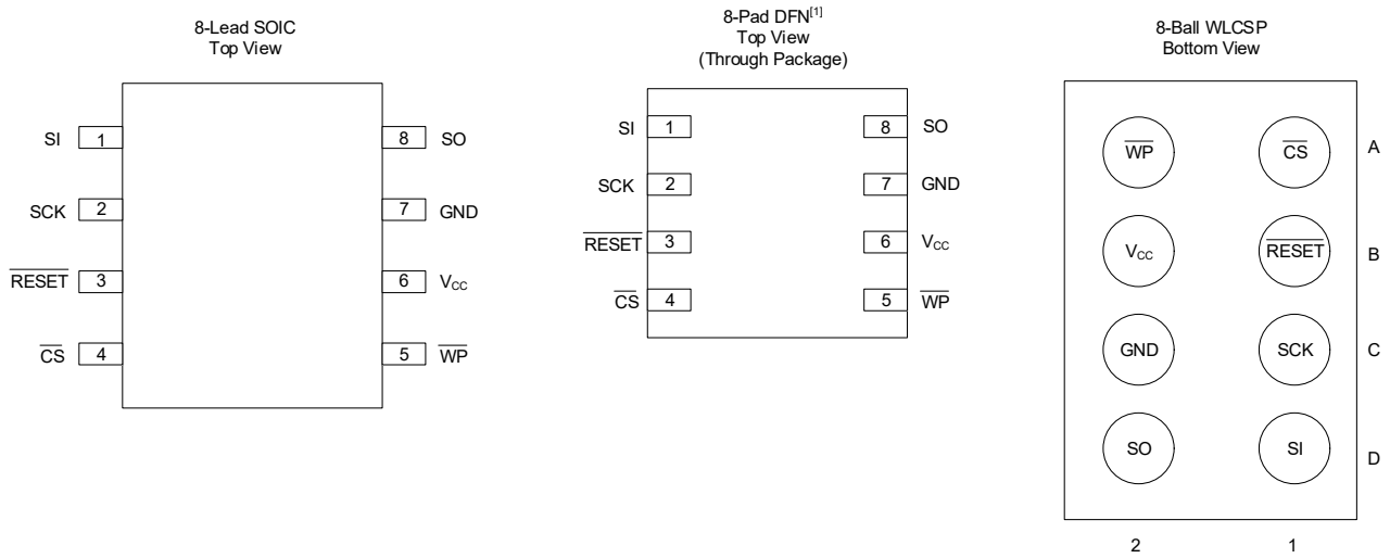
Figure 1. Pinouts
