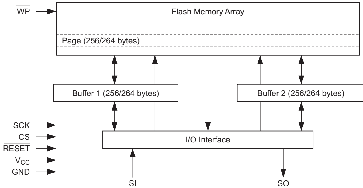
Figure 34. Block Diagram
