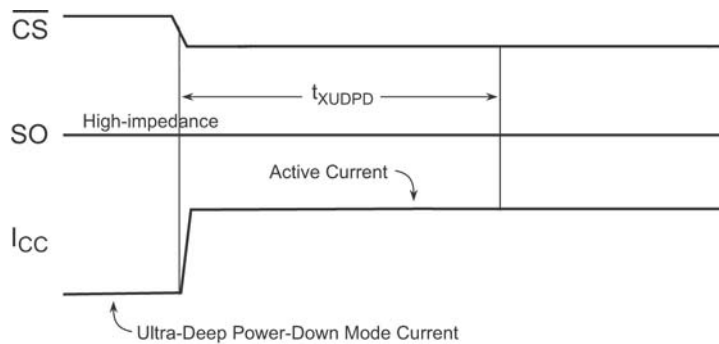
Figure 20. Exit Ultra-Deep Power-Down (Chip Select Low)
