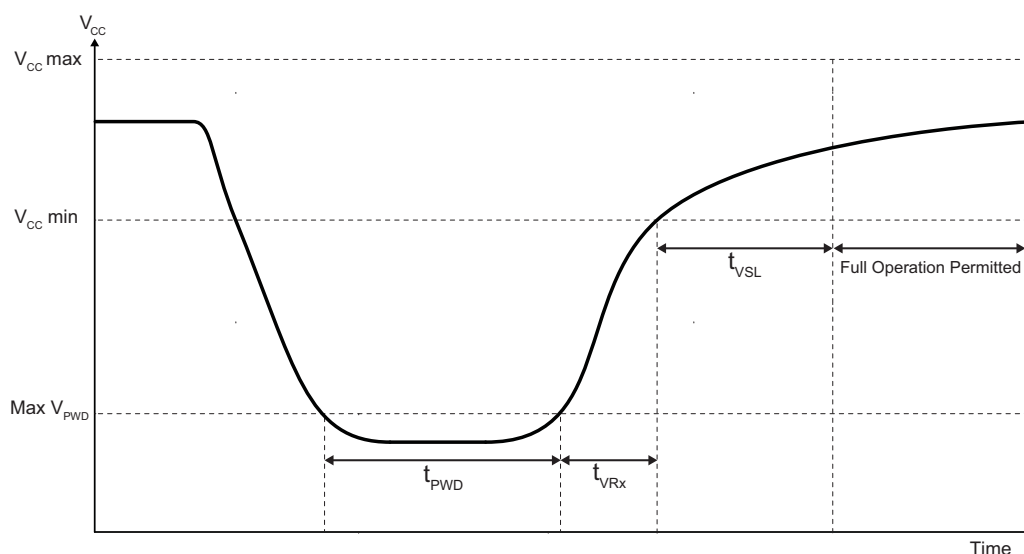
Figure 34. AC Power-up Timing After a Brown-Out
