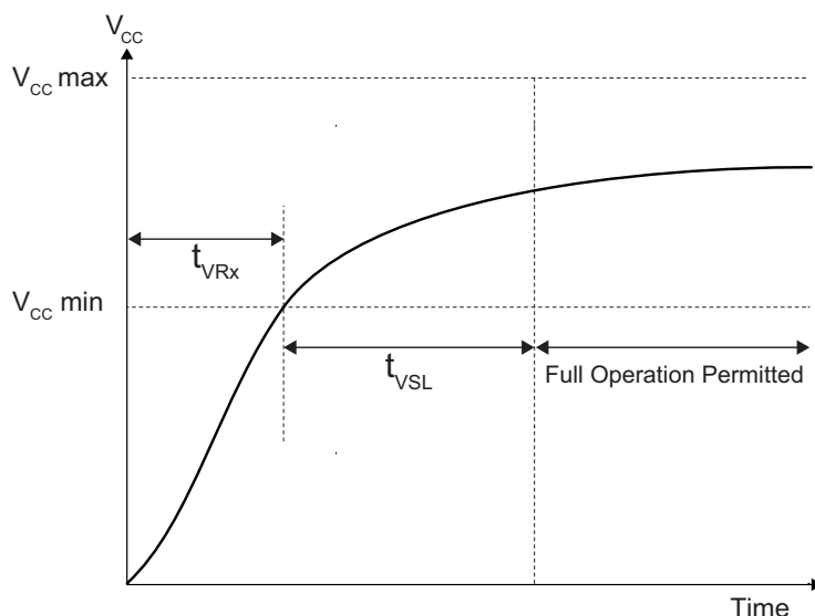
Figure 33. AC Timing During Device Power-Up
