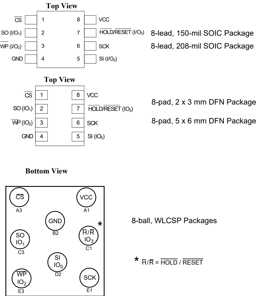
Figure 1. Memory Package Types
