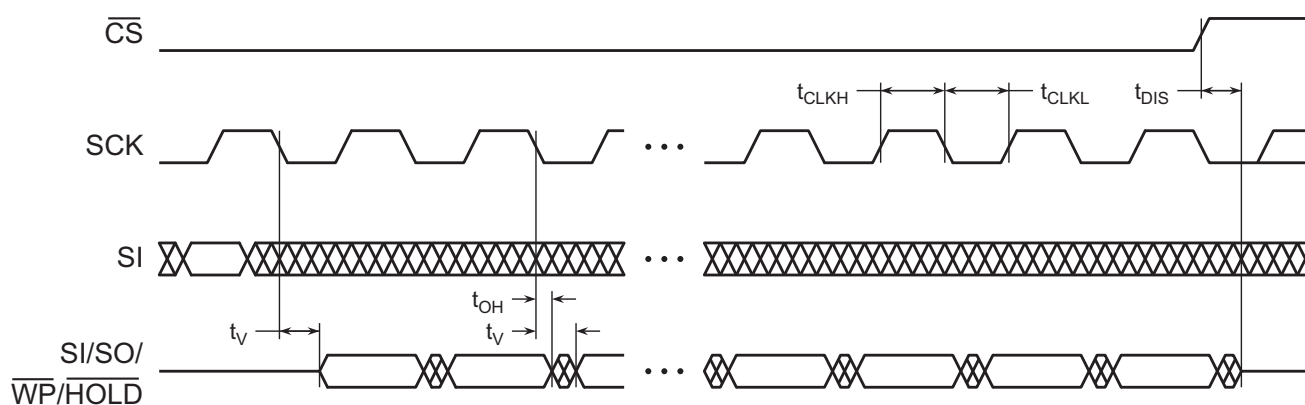
Figure 36. Serial Output Timing
