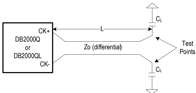
Figure 1. AC/DC Test Load for High Impedance Receivers
