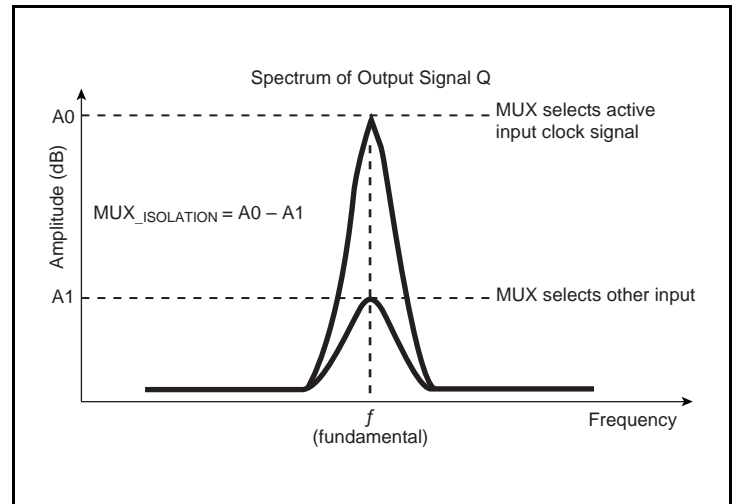
MUX Isolation
