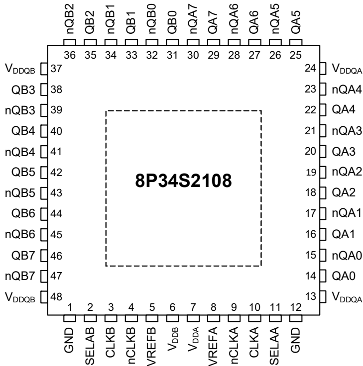
Figure 1. Pin Assignments for 7mm x 7mm 48-VFQFPN Package – Top View
