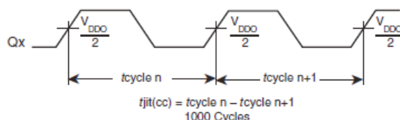
CYCLE-TO-CYCLE JITTER
