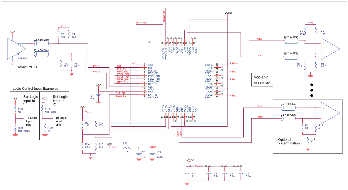
FIGURE 6. 873991-147 SCHMATIC LAYOUT
