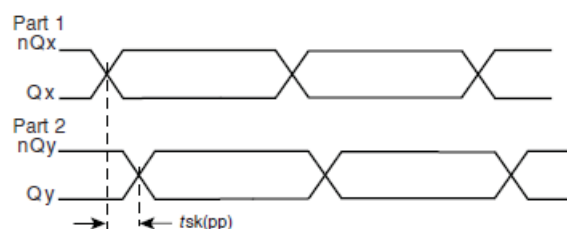
PART-TO-PART SKEW
