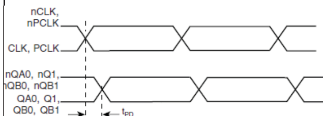
PROPAGATION DELAY
