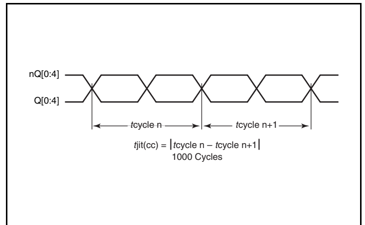
Cycle-to-Cycle Jitter
