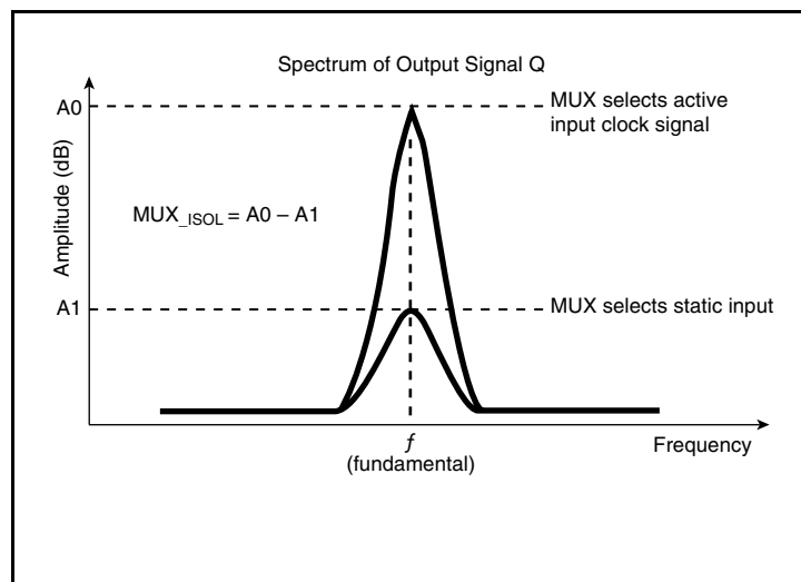
MUX Isolation
