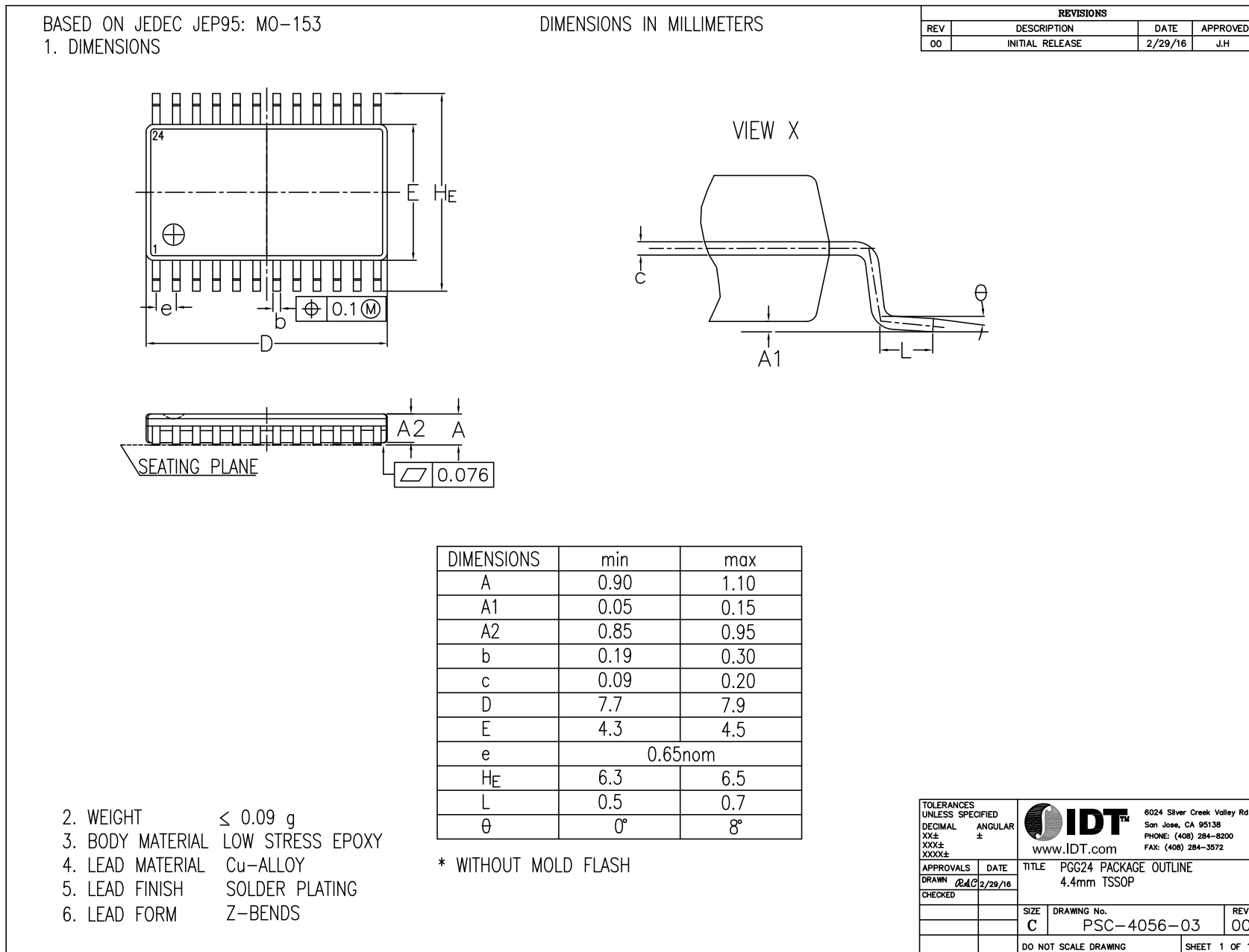
Package Drawings Figure 27. Package Drawings
