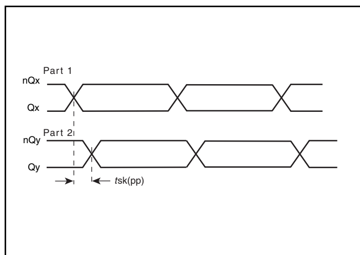
Part-to-Part Skew
