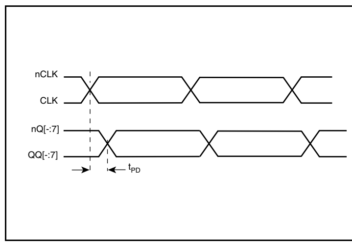
Propagation Delay
