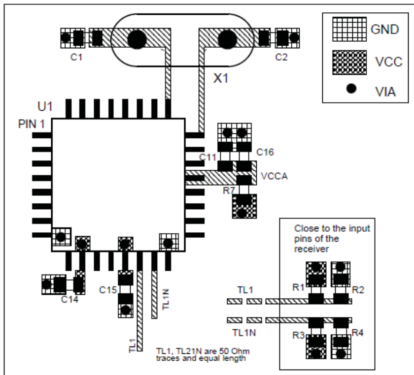
FIGURE 7B. PCB BOARD LAYOUT FOR 8430-61
