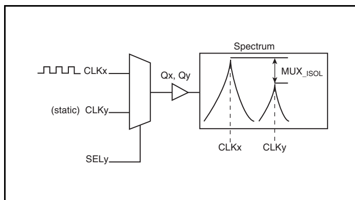
MUX Isolation
