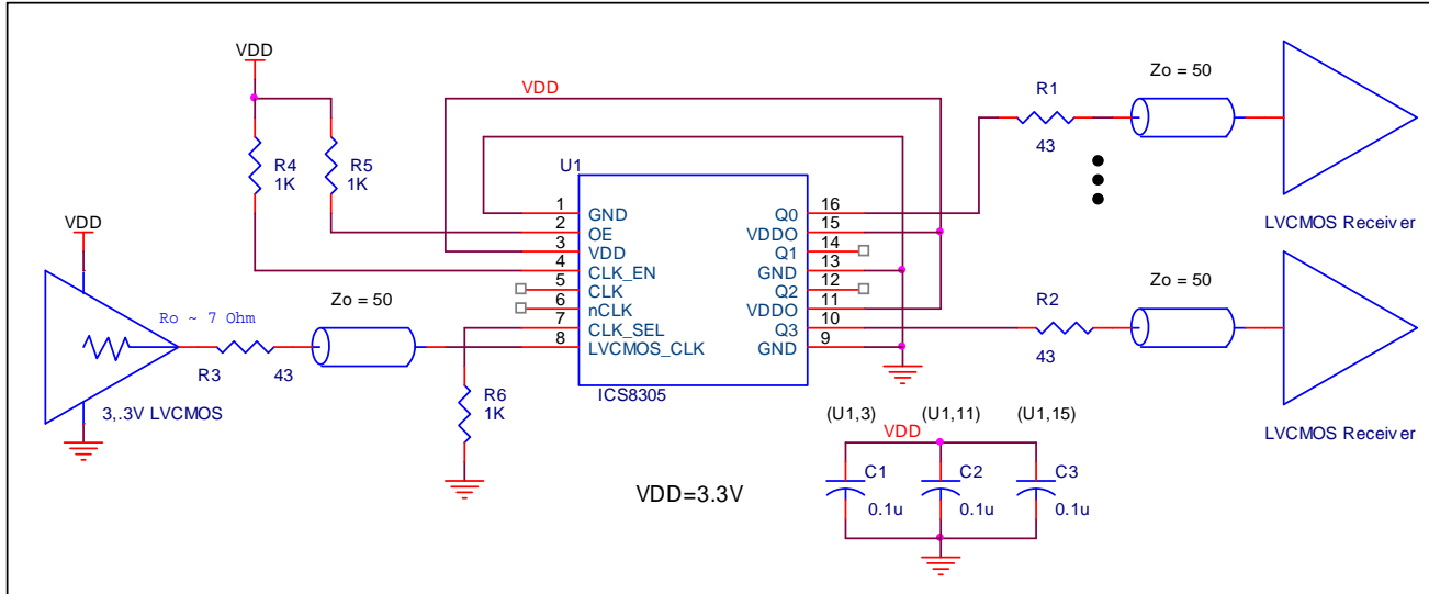
Figure 4. ICS8305 LVC MOS Clock Output Buffer Schematic Example
