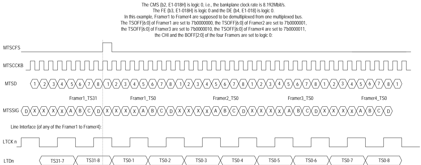
Figure 46. E1 Transmit Multiplexed Mode - Functional Timing Example 1
