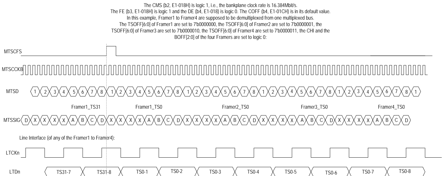
Figure 47. E1 Transmit Multiplexed Mode - Functional Timing Example 2
