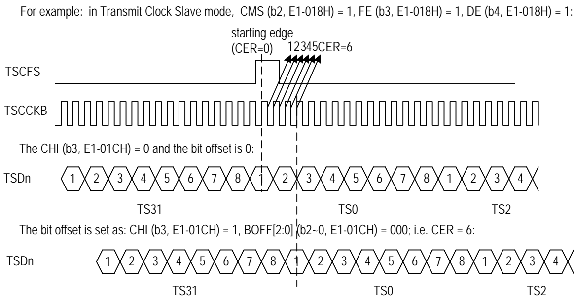
Figure 51. Transmit Bit Offset in E1 Mode - 4
