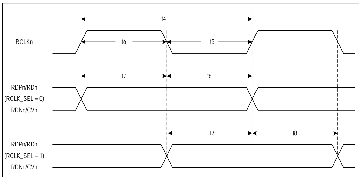
Figure-26 Receive System Interface Timing
