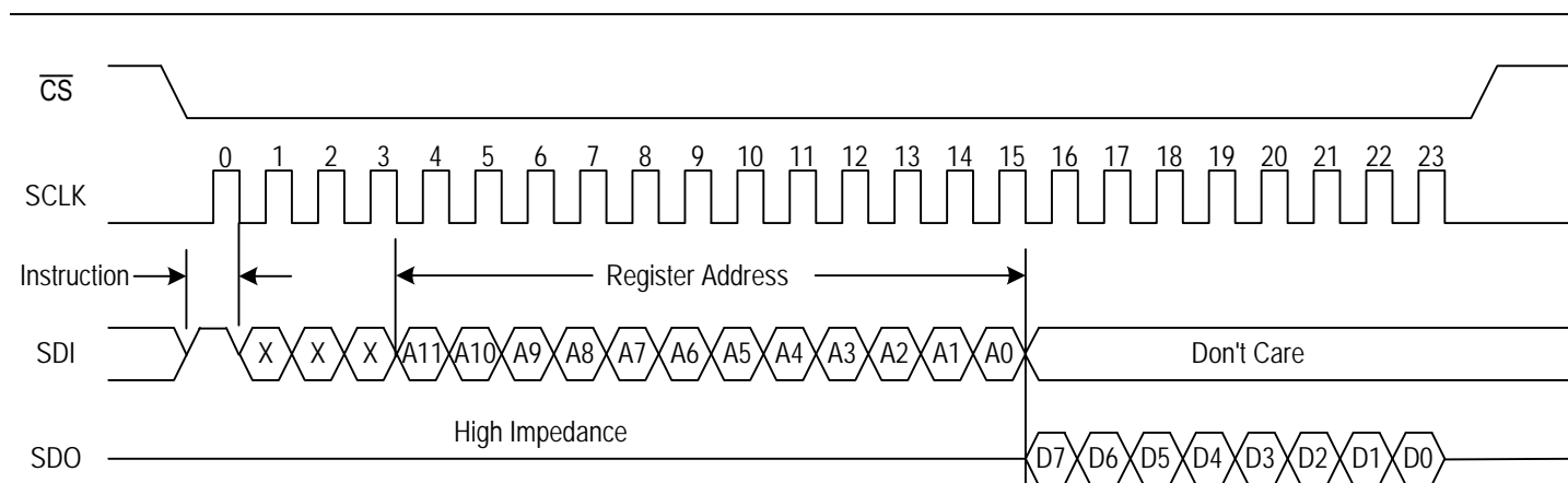
Figure-21 Read Operation In SPI Mode
