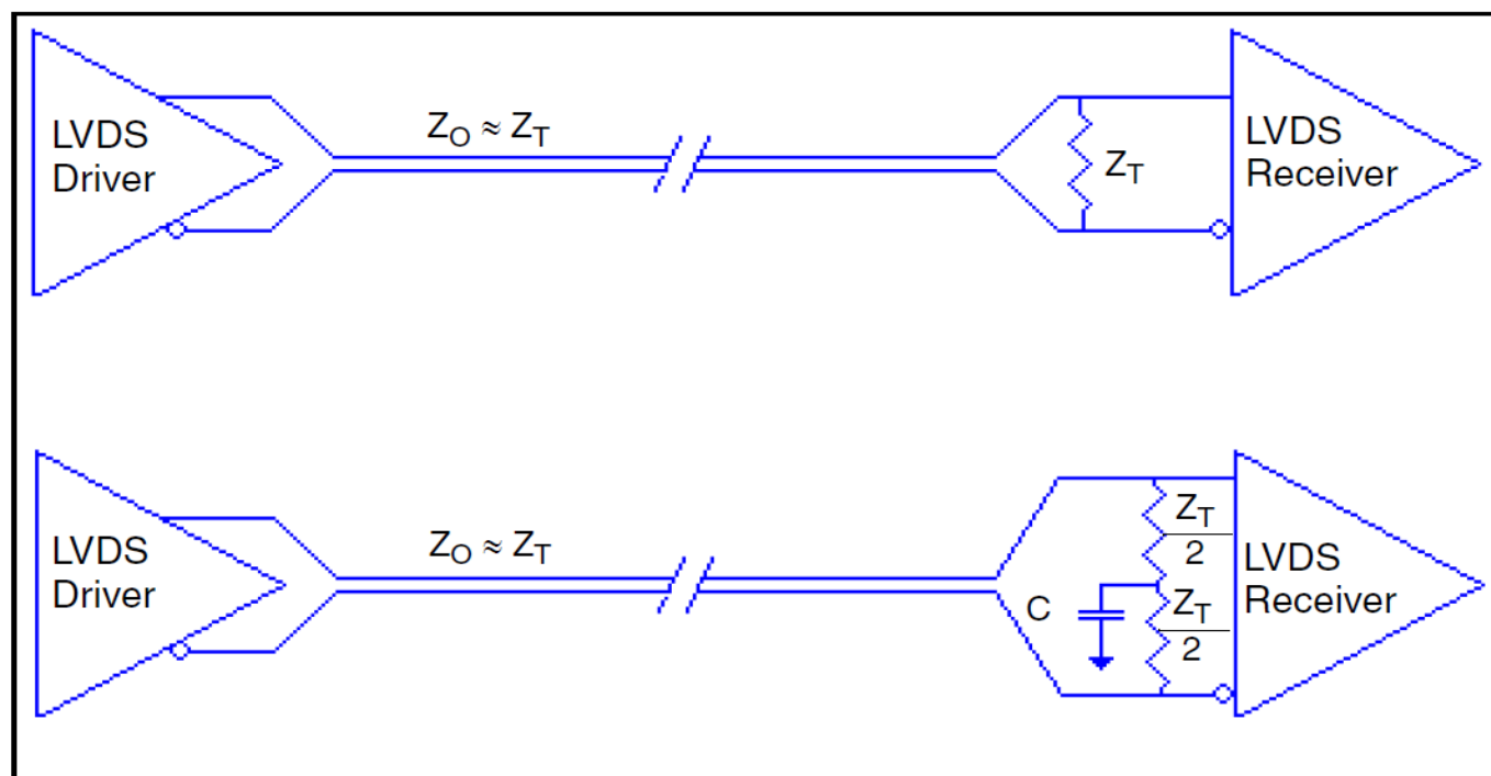
Figure 43. Recommended LVDS Output Port Line Termination
