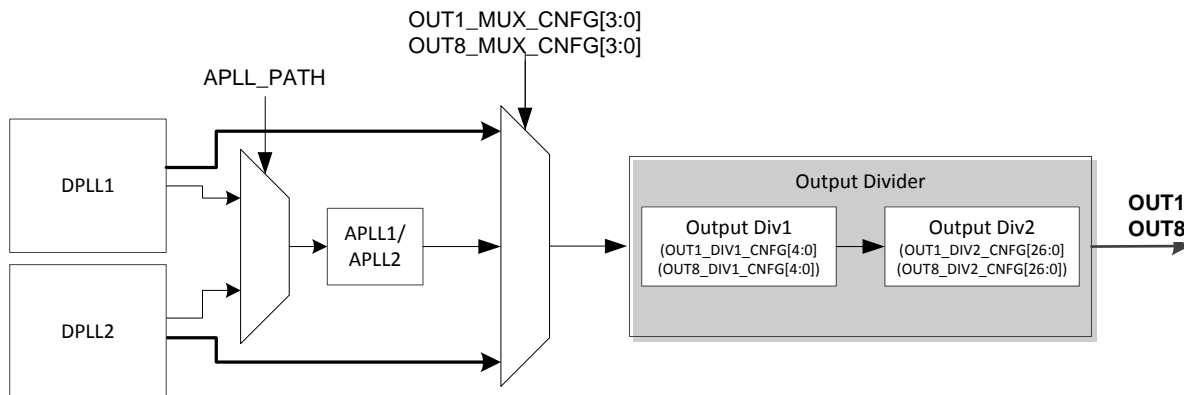
Figure 21. OUT1 and OUT8 output dividers
