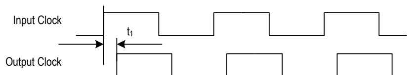
Figure 45. Input / output clock timing
