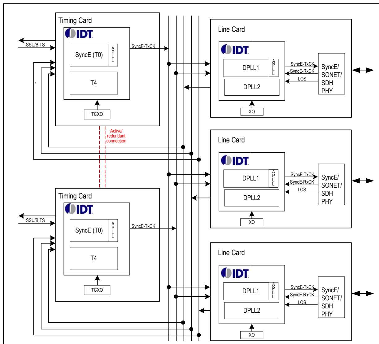
Figure 9. SyncE/SONET/SDH active/redundant application
