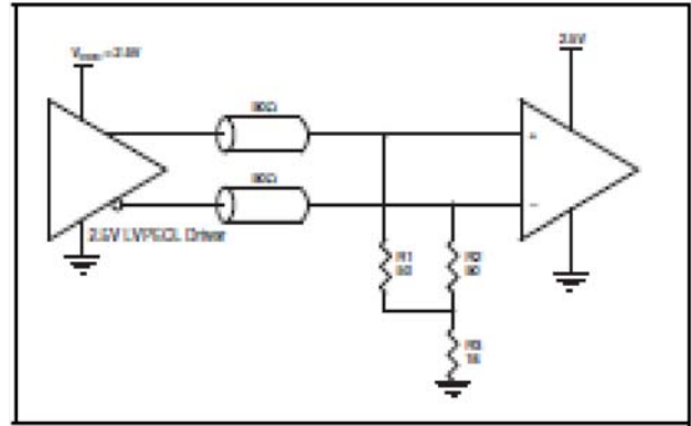
Figure 40. 2.5V LVPECL Output Termination
