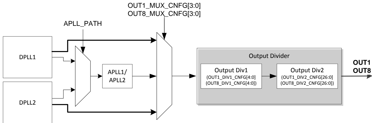
Figure 21. OUT1 and OUT8 output dividers
