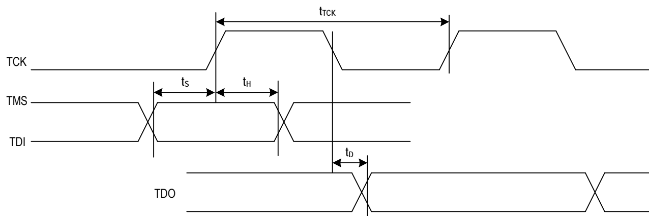
Figure 30. JTAG Interface Timing Diagram
