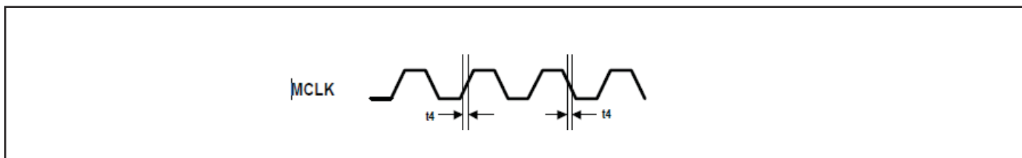
Figure 2. MCLK Timing
