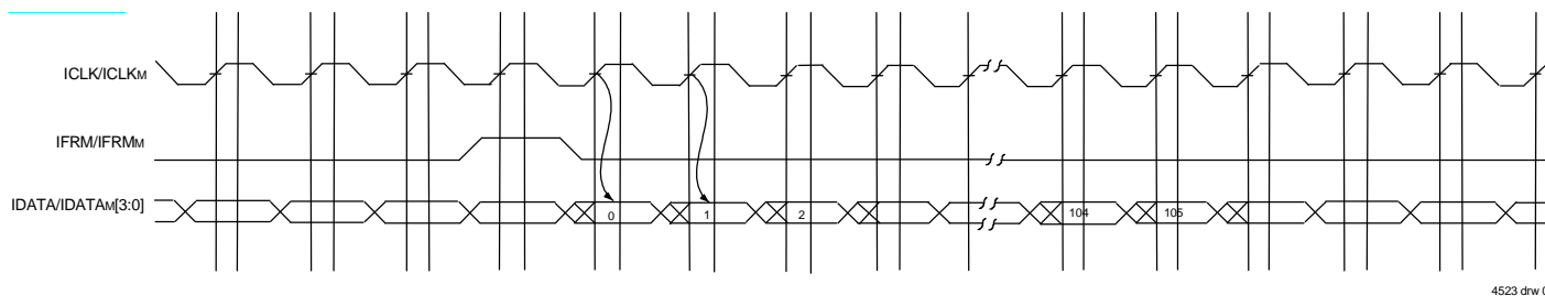
Figure 5 One Cell Transfer on Receive DPI Bus
