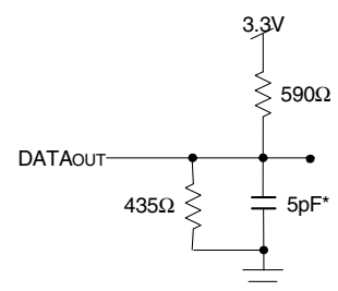
Figure 2. Output Test Load (for t LZ , t HZ , t wZ , t owZ )
