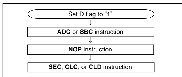
Fig. 3 Execution of decimal calculations
