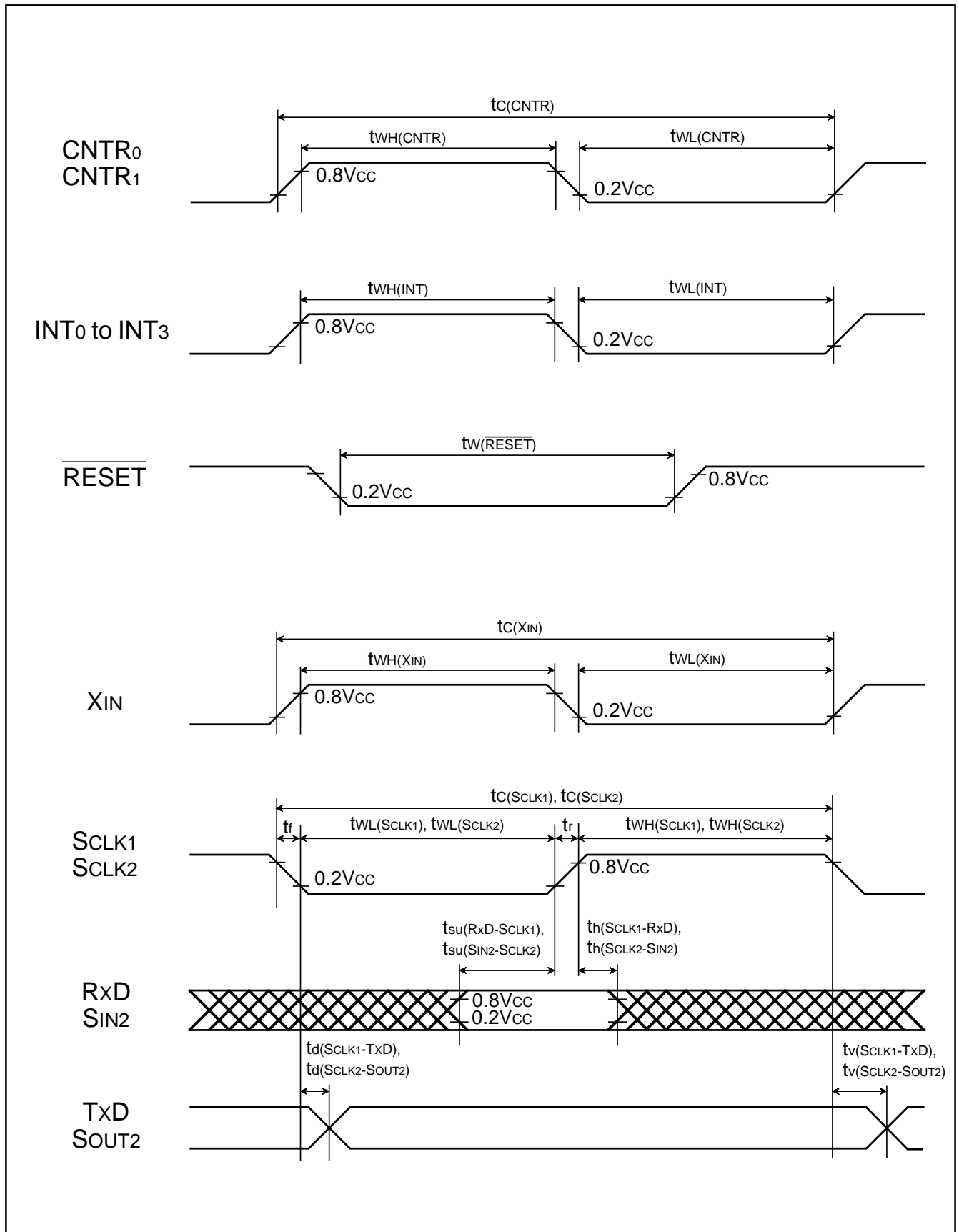
Fig. 69 Timing diagram
