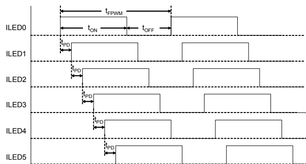
FIGURE 24. PHASE SHIFT WITH 7-BIT PROGRAMMABLE DELAY
