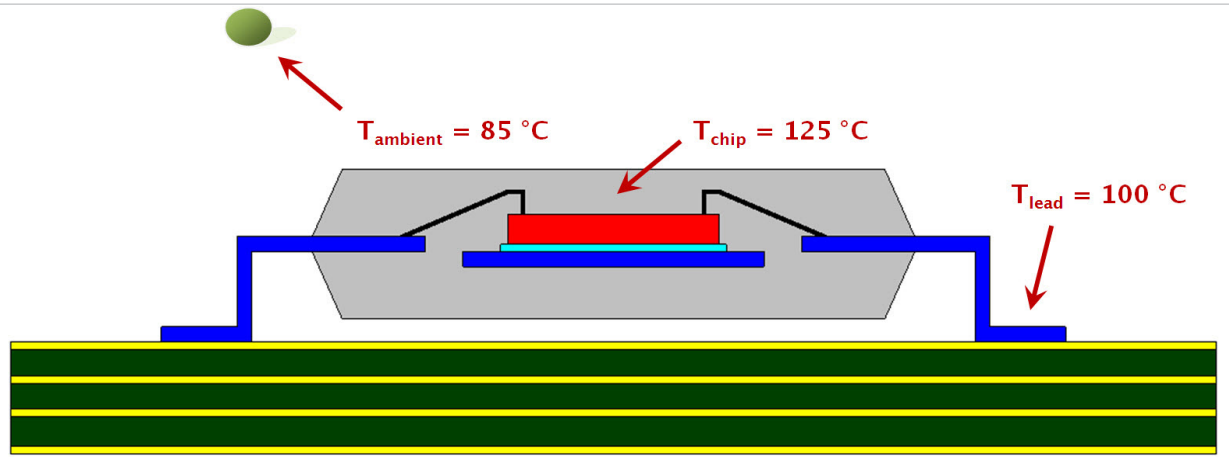
Figure 1: Package on a PCB with relevant temperature-monitor points
