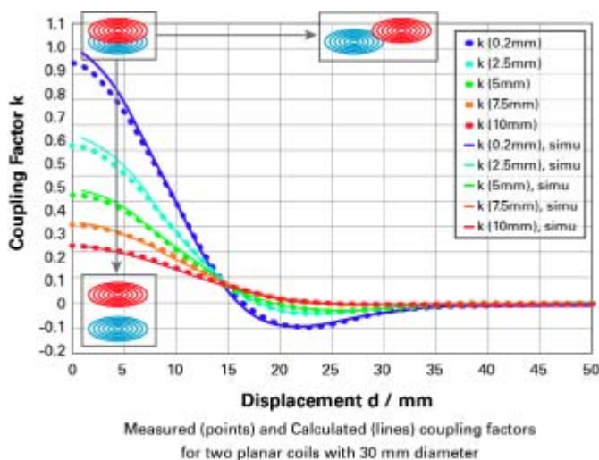
Figure 2: Coupling Displacement
