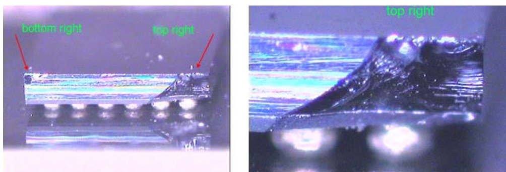
Figure 7. Mechanical Damage to WLCSP Device Due to Improper Handling
