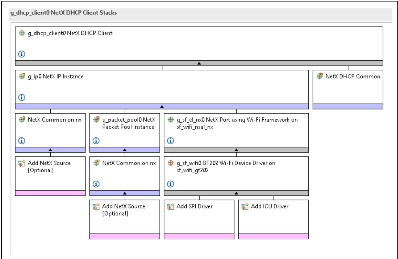
Figure 6. Adding SPI Driver and IRQ Driver
