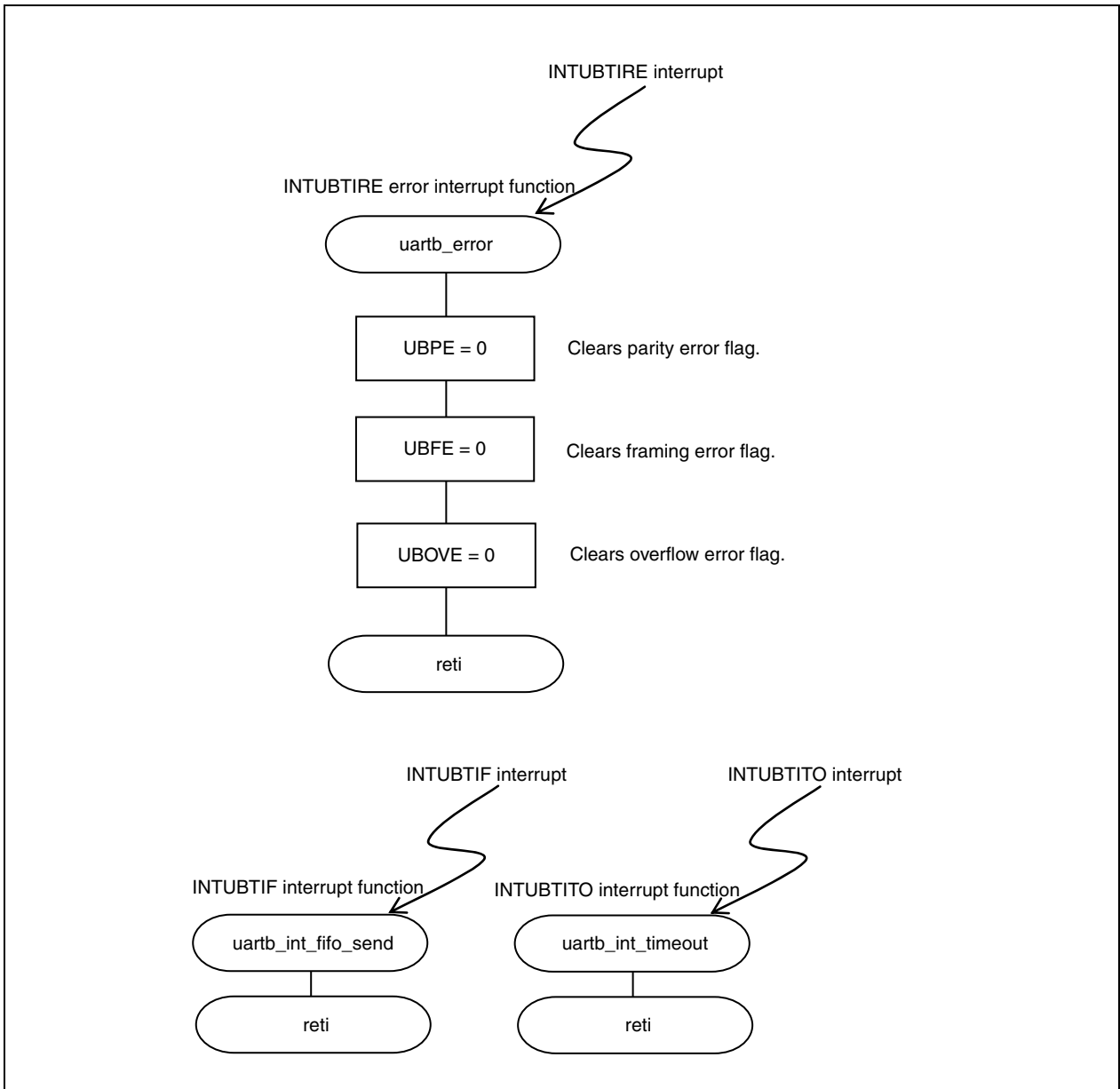
Figure 2-1. FIFO Mode (4/4)
