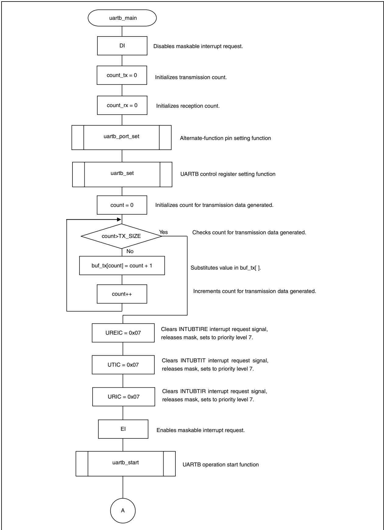
Figure 1-1. Single Mode (1/4)
