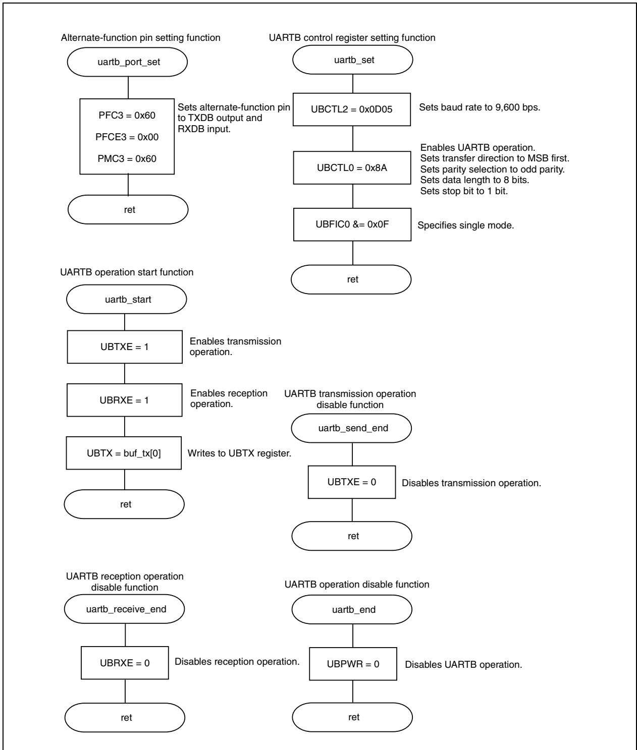
Figure 1-1. Single Mode (3/4)
