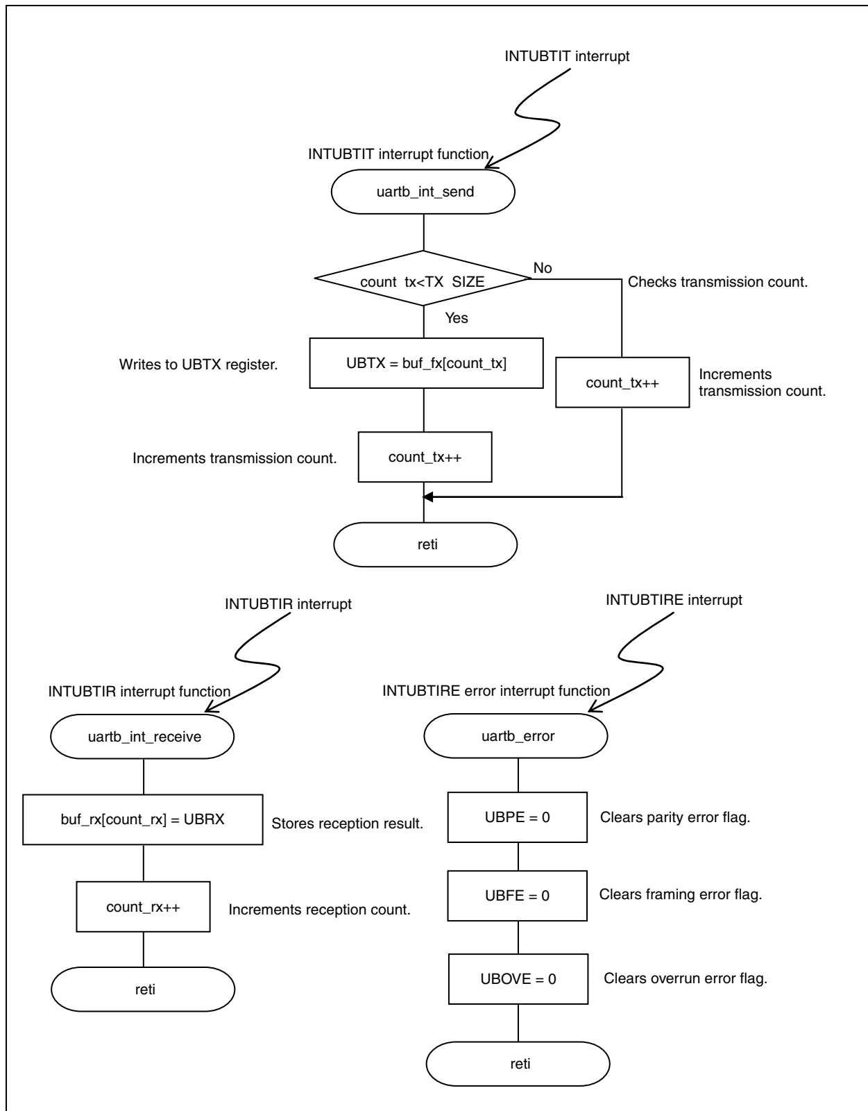
Figure 1-1. Single Mode (4/4)
