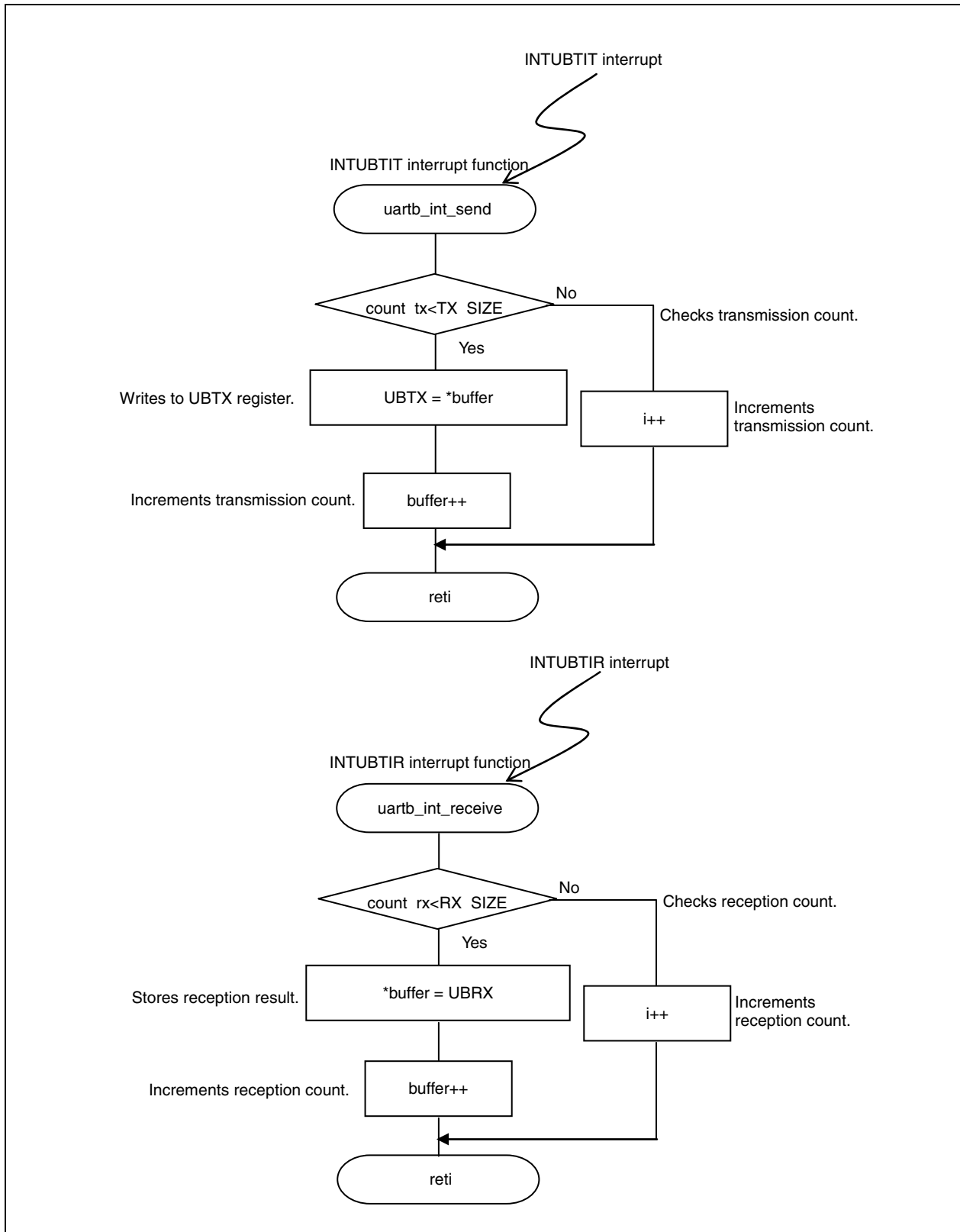
Figure 2-1. FIFO Mode (3/4)
