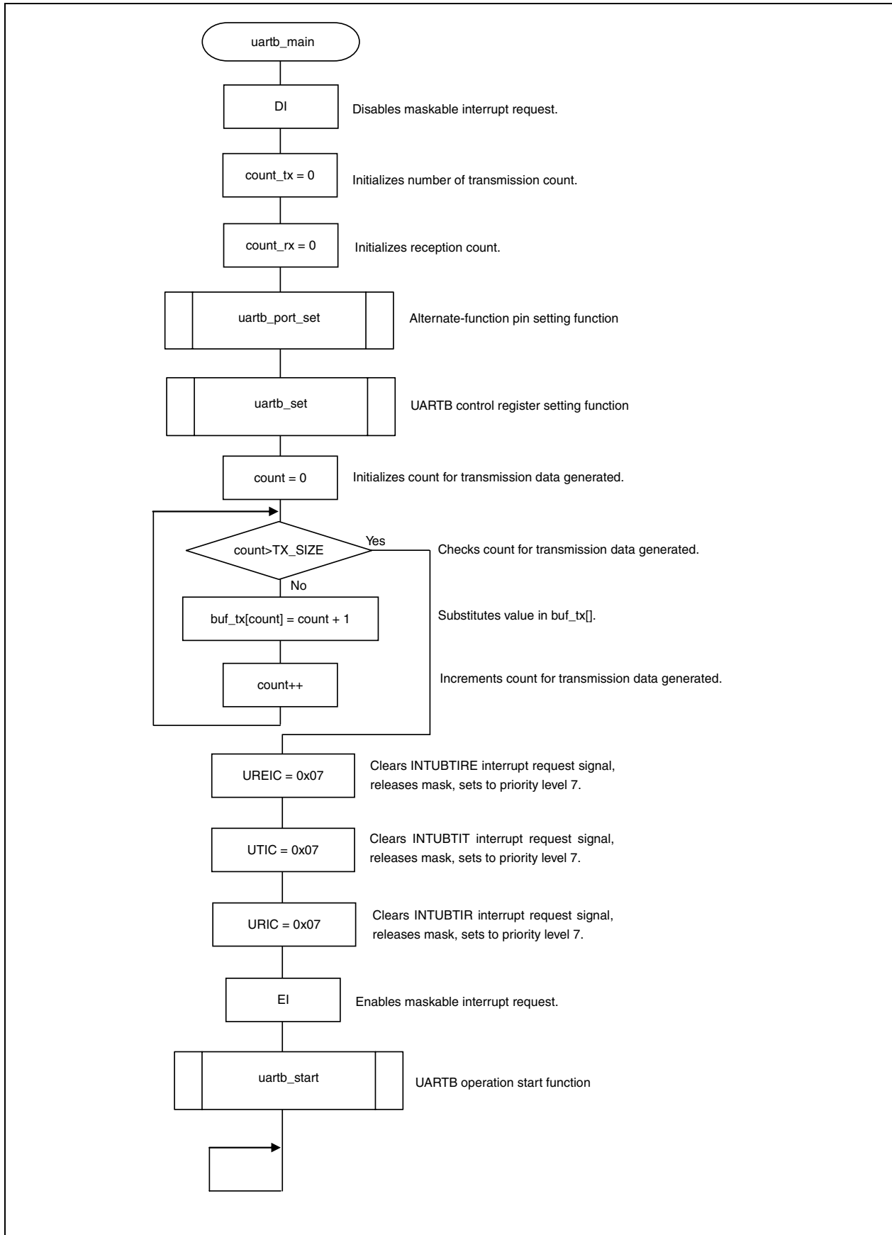
Figure 2-1. FIFO Mode (1/4)
