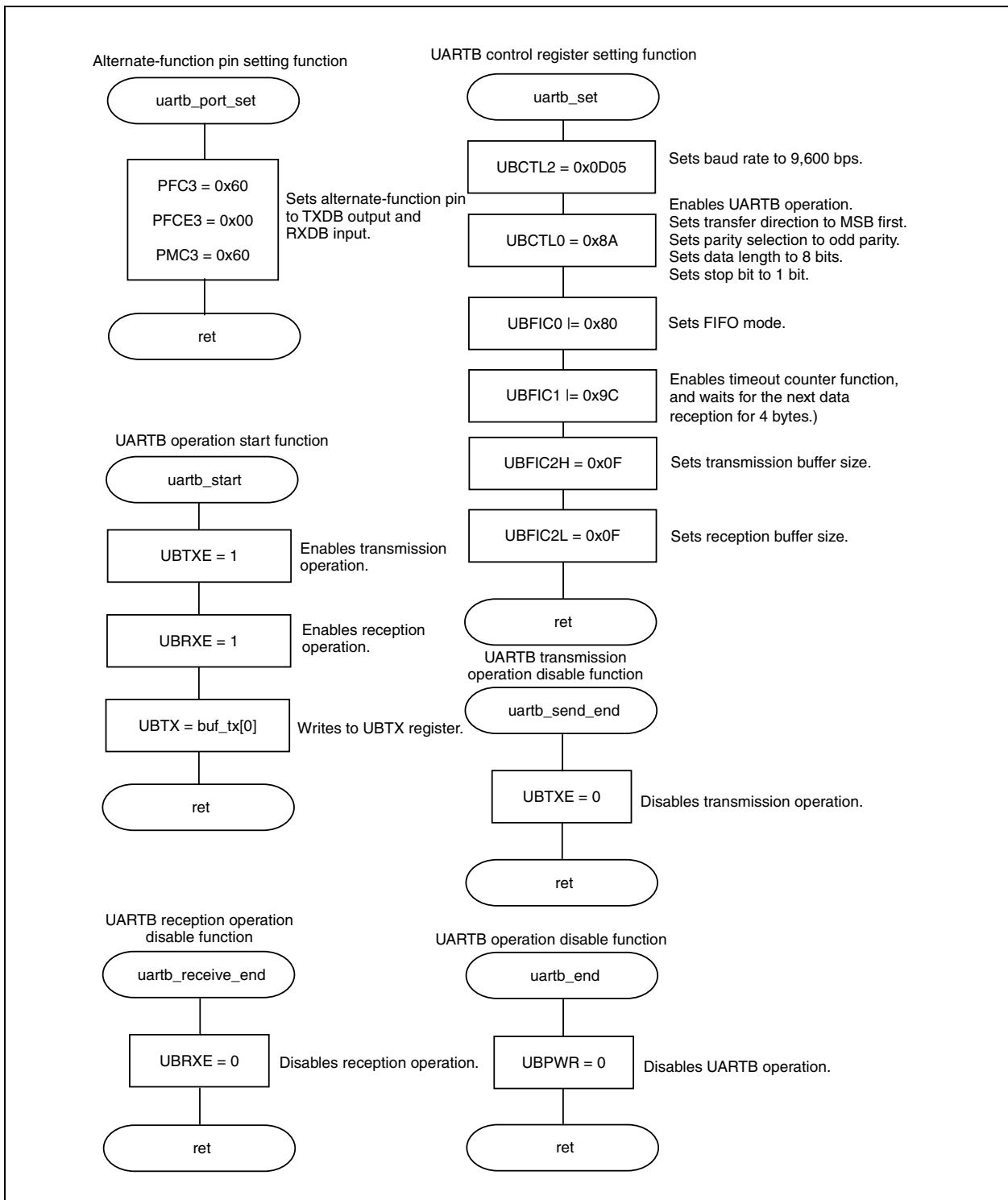
Figure 2-1. FIFO Mode (2/4)
