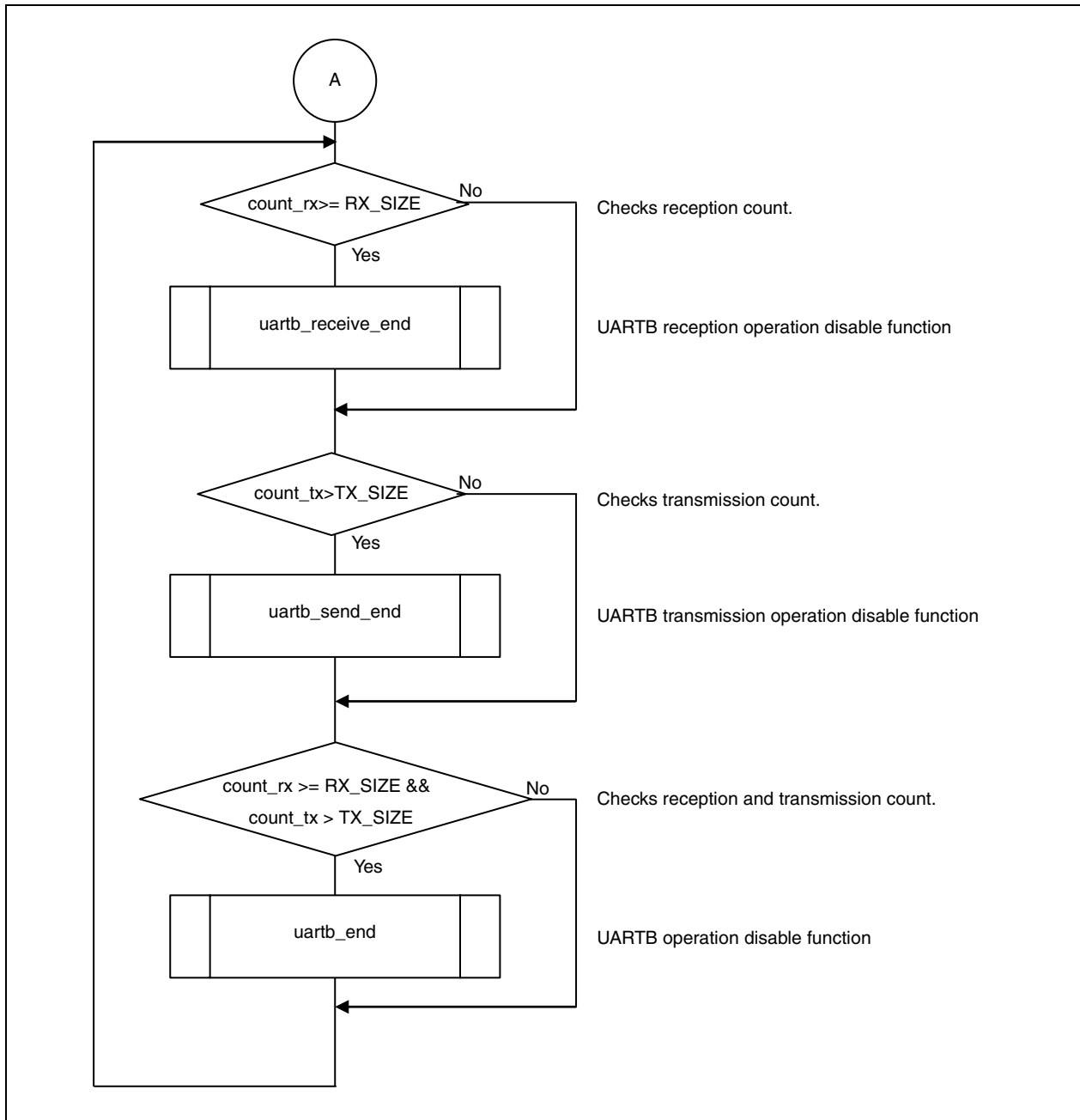
Figure 1-1. Single Mode (2/4)
