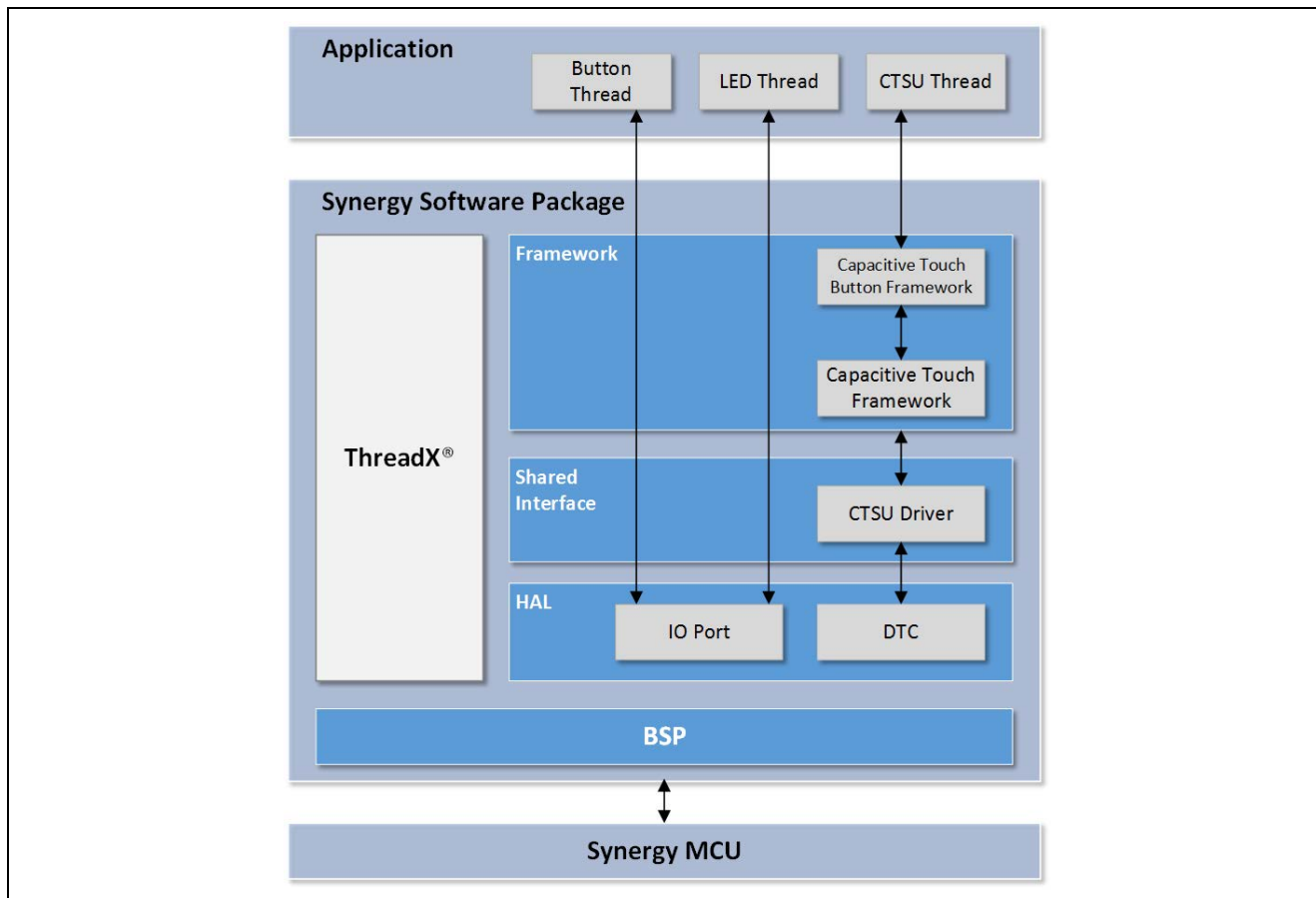
Figure 2. Button/CTSU Application Software Architecture
