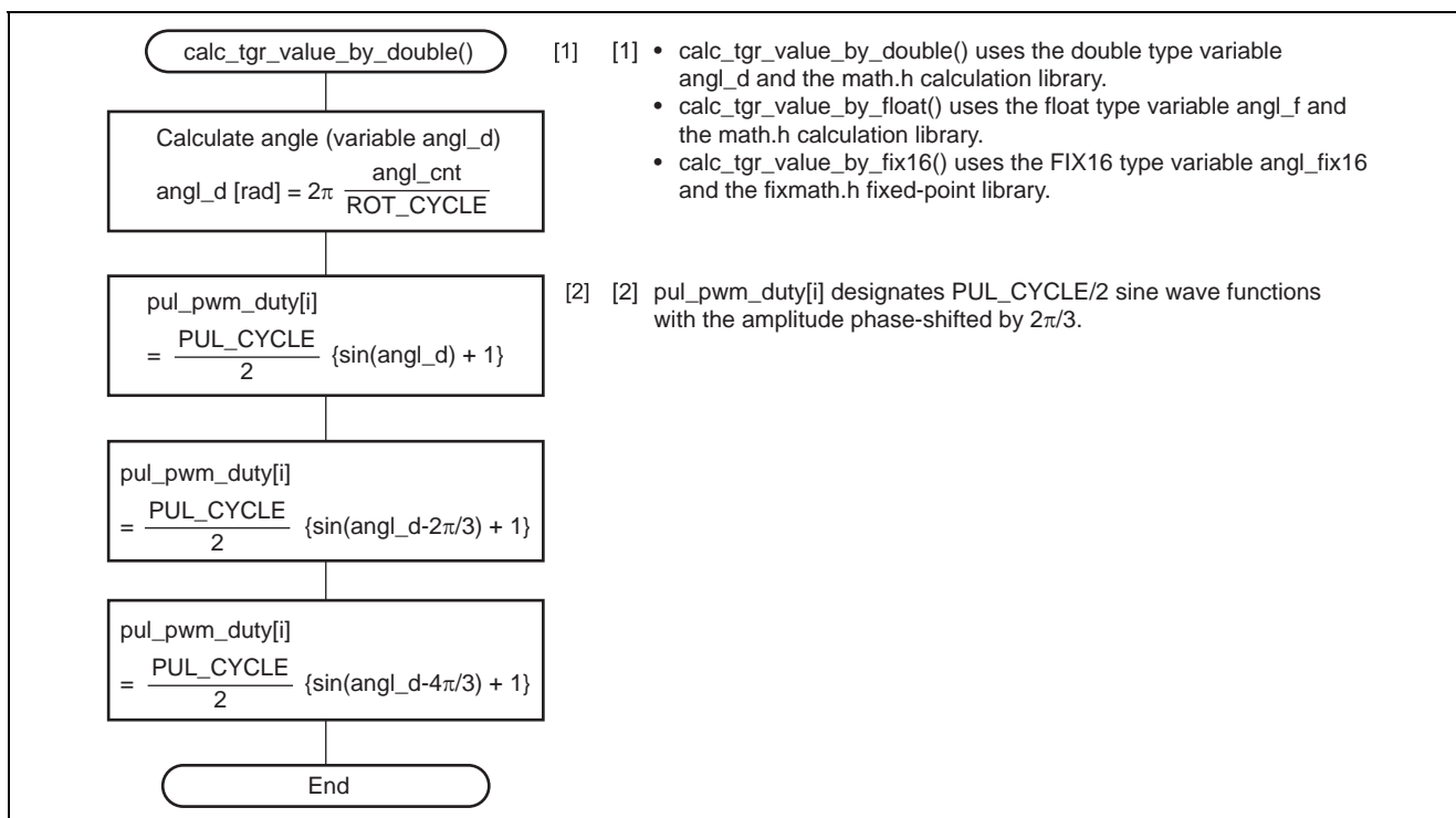
Figure 17 Calculation of Compare Register Values
