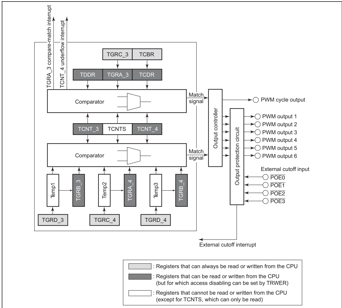
Figure 3 Block Diagram of Channels 3 and 4 in Complementary PWM Mode
