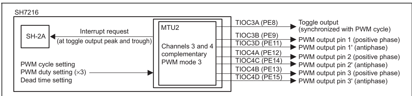
Figure 1 Three-Phase Complementary PWM Output (Complementary PWM Mode 3)
