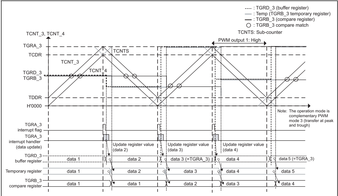
Figure 7 PWM Duty Update Timing (PWM Output 1)
