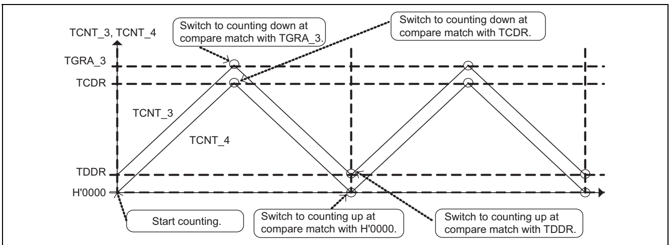
Figure 5 Operation of Timer Counters
