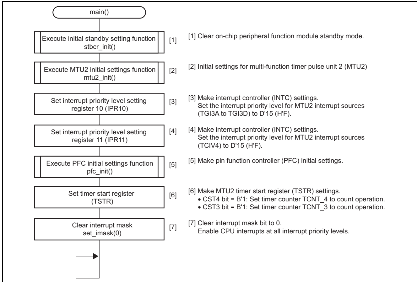
Figure 11 Processing by Function main
