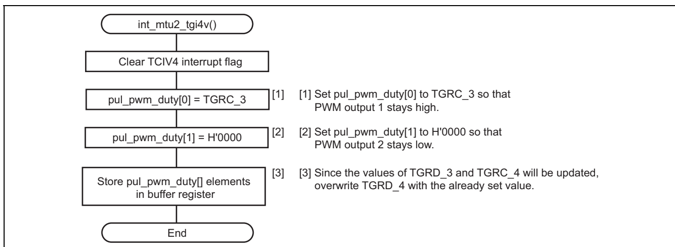
Figure 16 MTU2 Overflow Interrupt (TCNT_4) Handler
