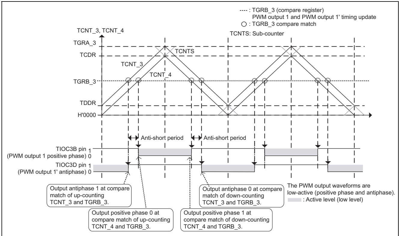
Figure 6 Complementary PWM Output Waveforms
