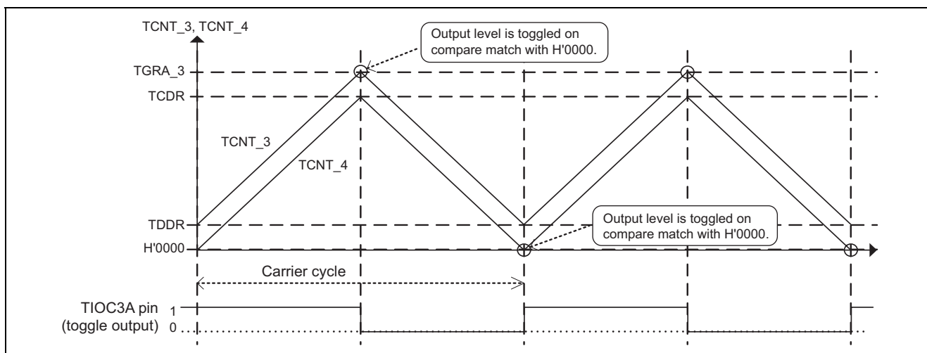
Figure 9 Operation for Toggling an Output in Synchronization with the PWM Cycle
