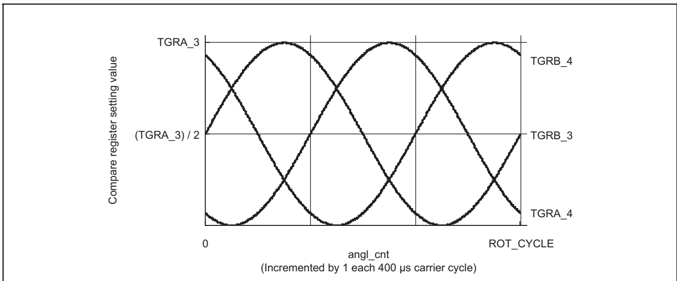
Figure 8 Setting Values of Compare Registers TGRB_3, TGRA_4, and TGRB_4
