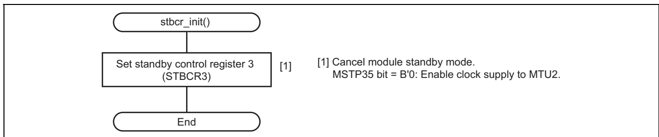
Figure 12 Initialization for Standby
