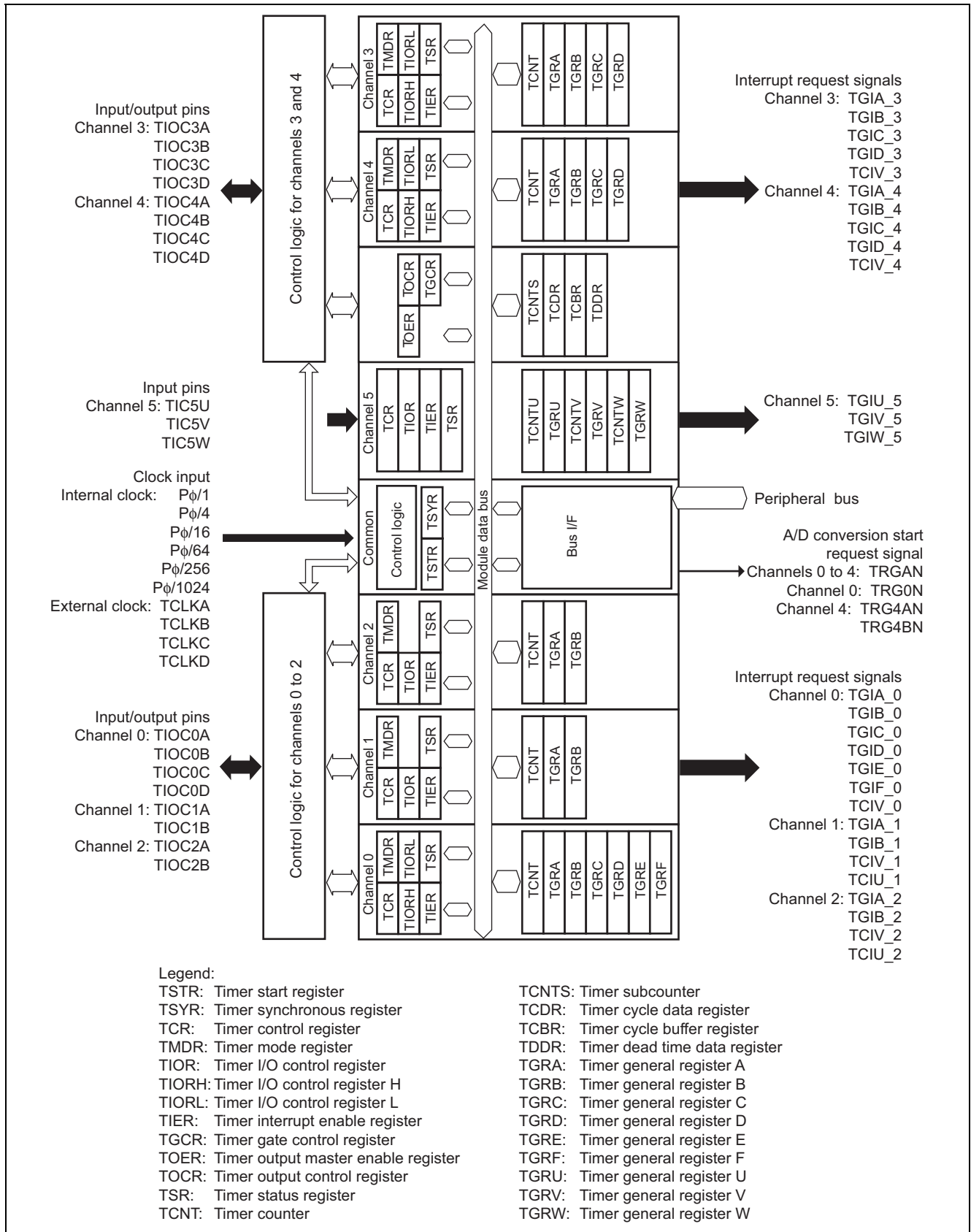
Figure 2 Block Diagram of MTU2
