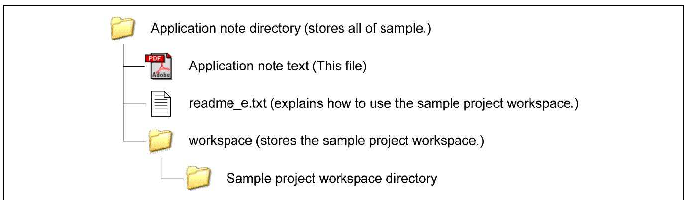
Figure 1.1 Directory Configuration
