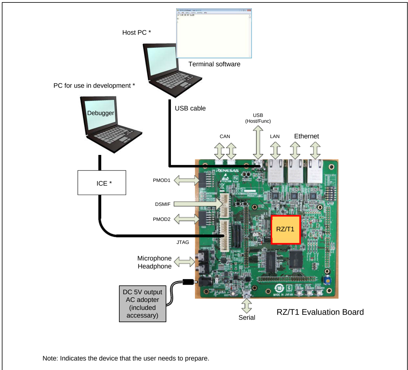
Figure 1.1 System Configuration
