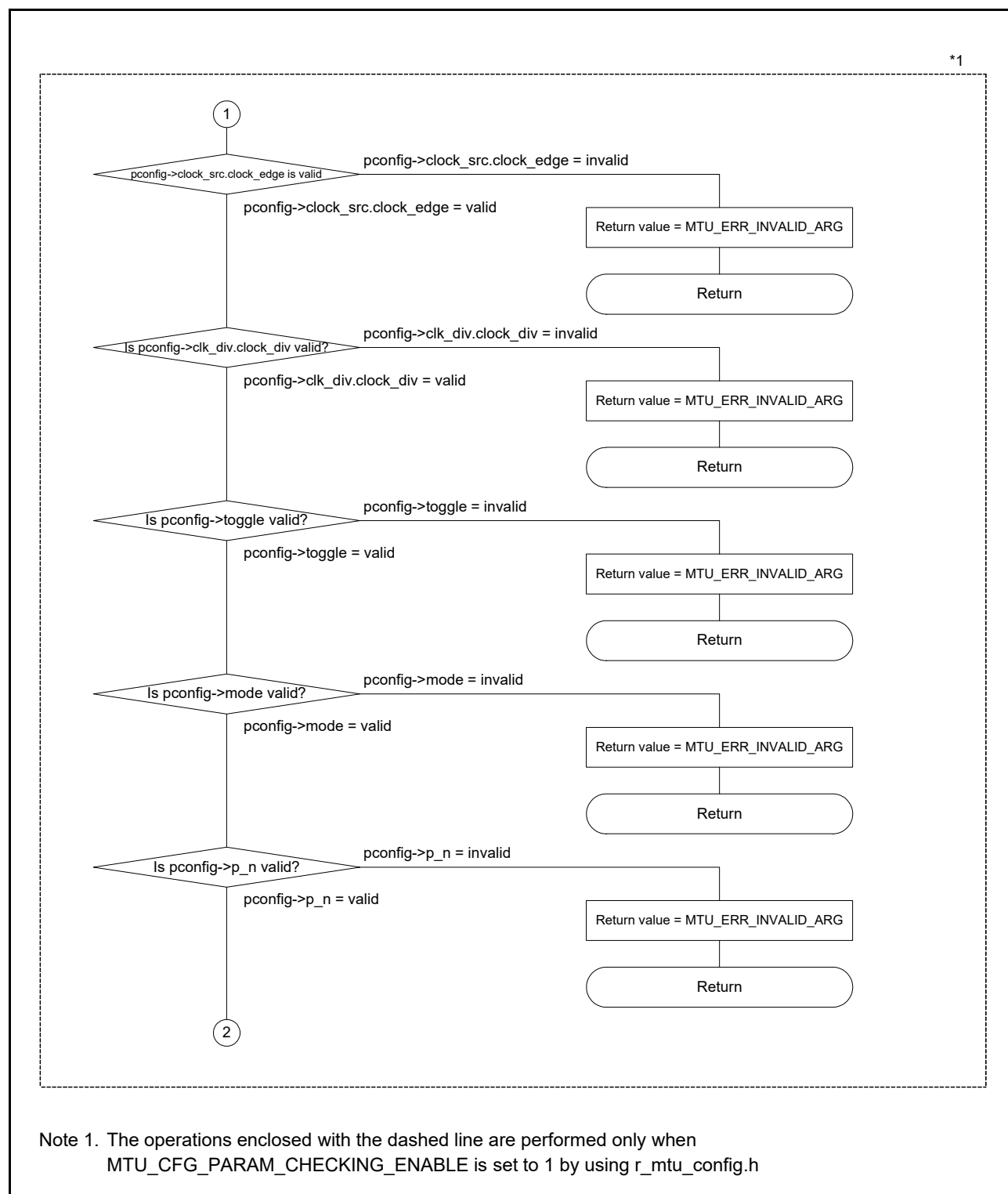
Figure 6.18 Complementary PWM Mode End Processing (2)
