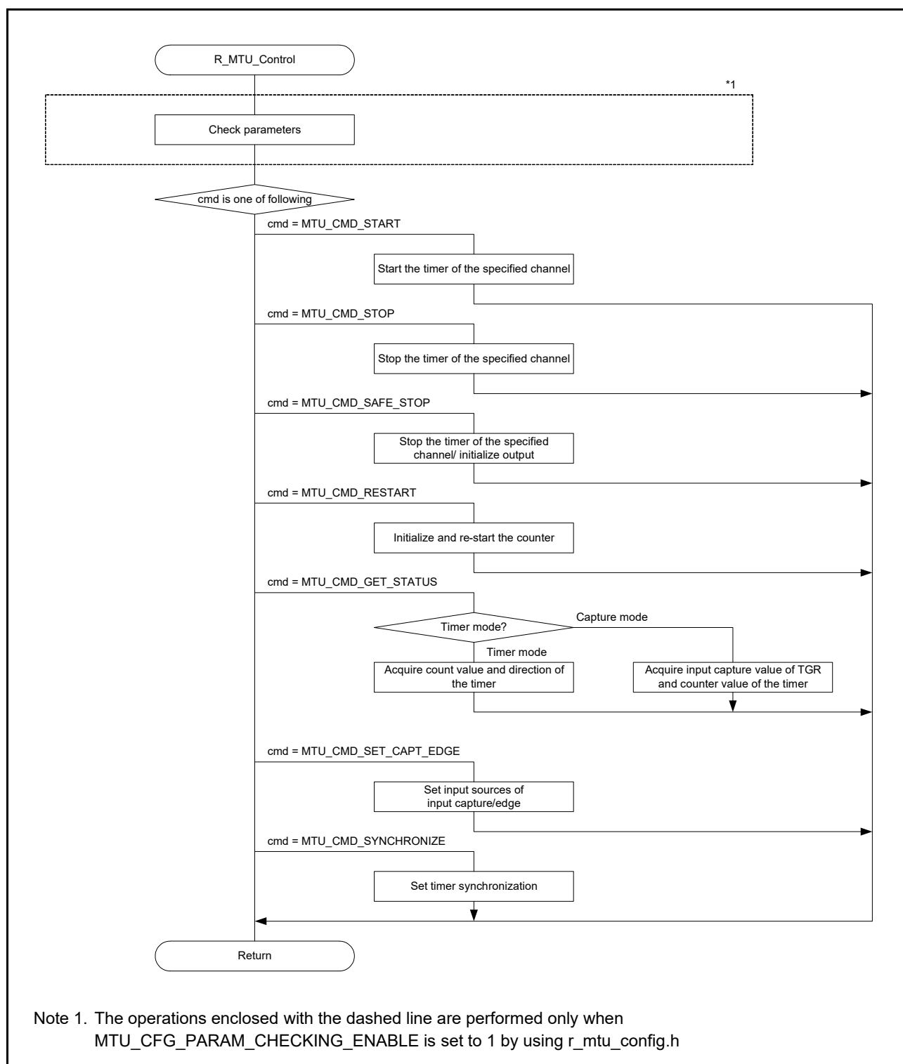
Figure 6.30 MTU Controlling
