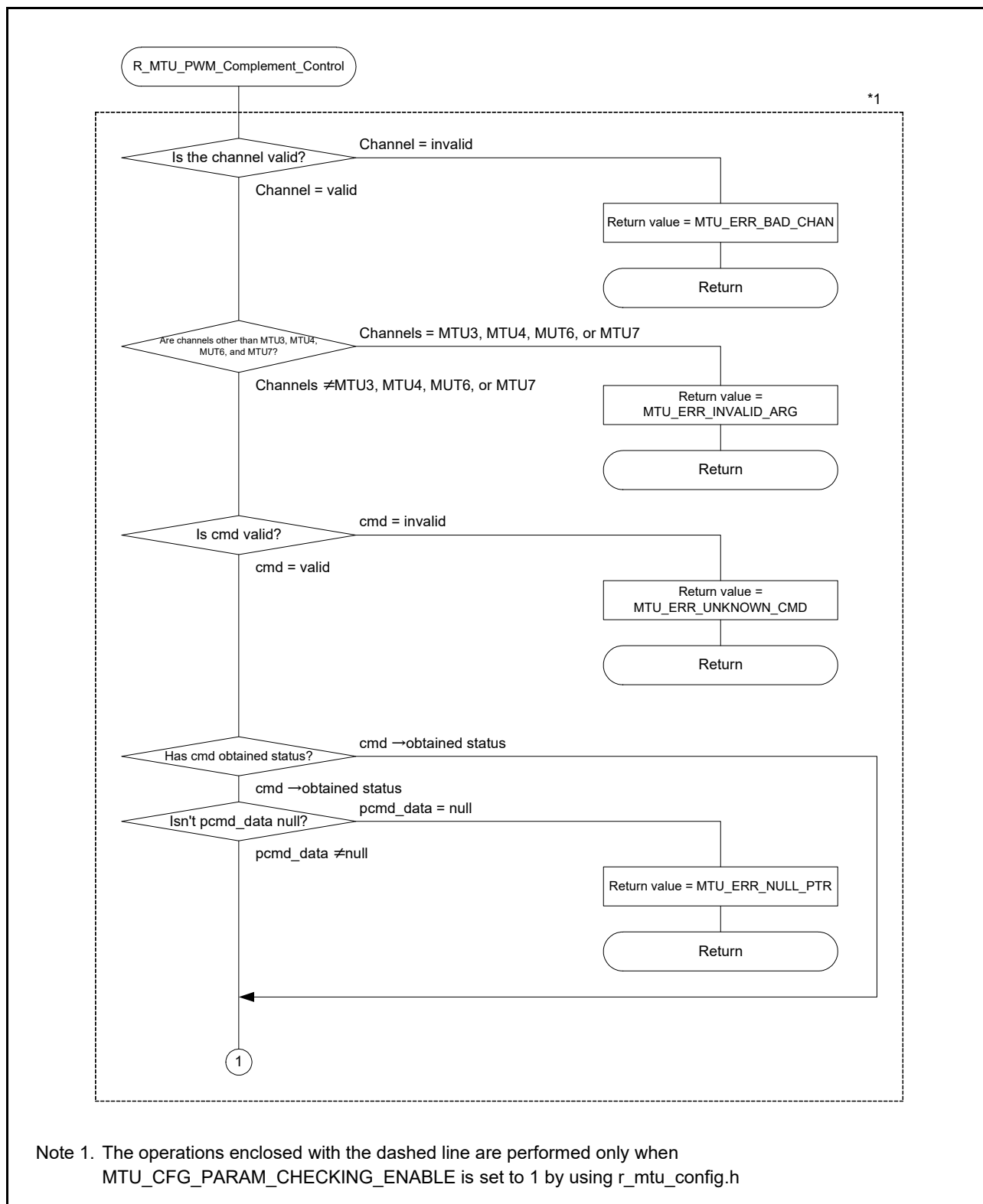
Figure 6.23 Complementary PWM Controlling (1)
