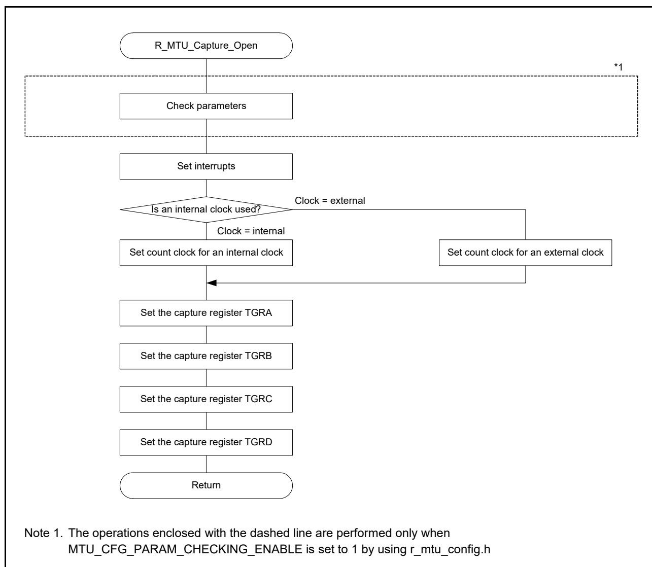
Figure 6.27 MTU Capture Processing
