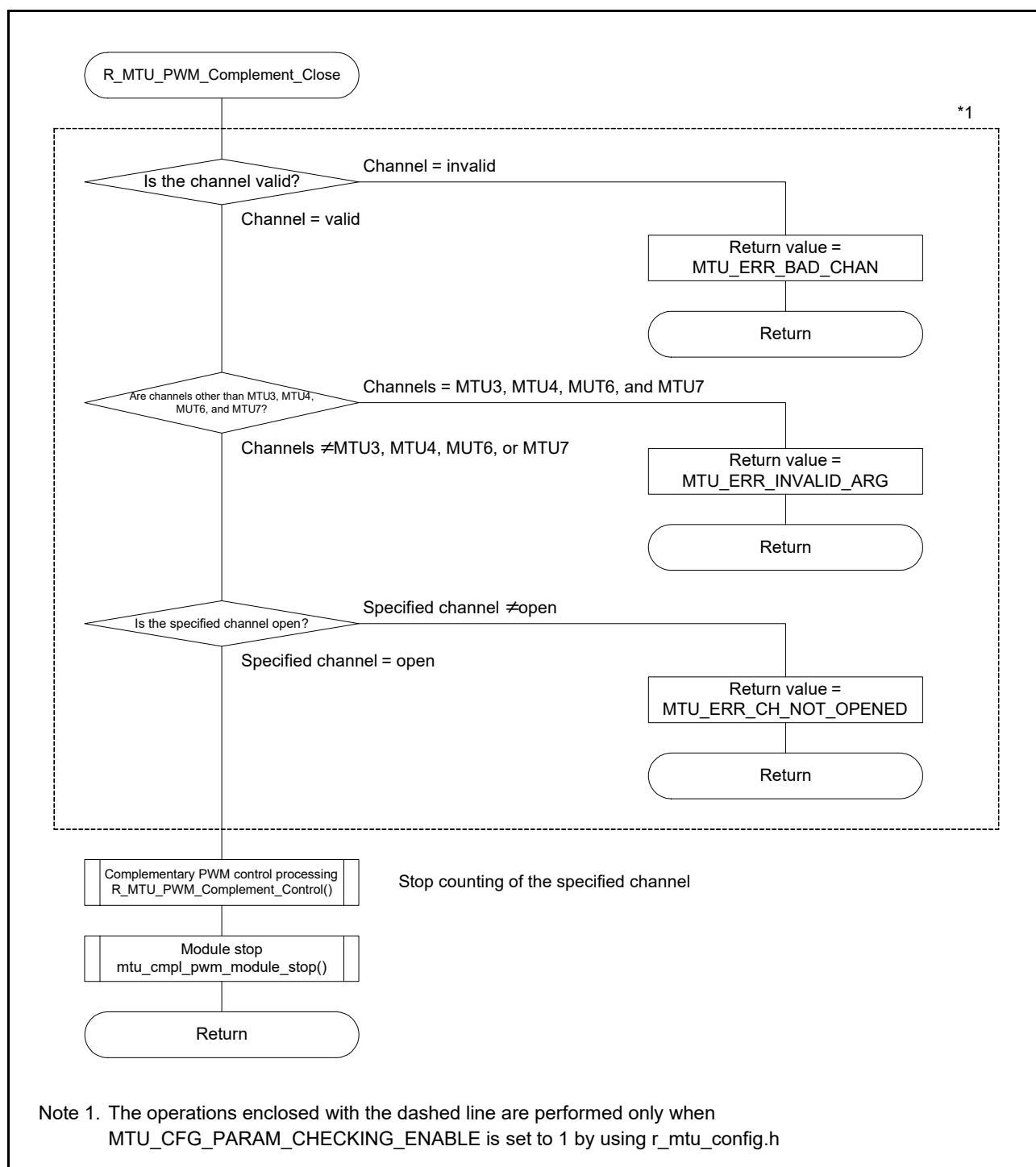
Figure 6.22 Complementary PWM Mode End Processing
