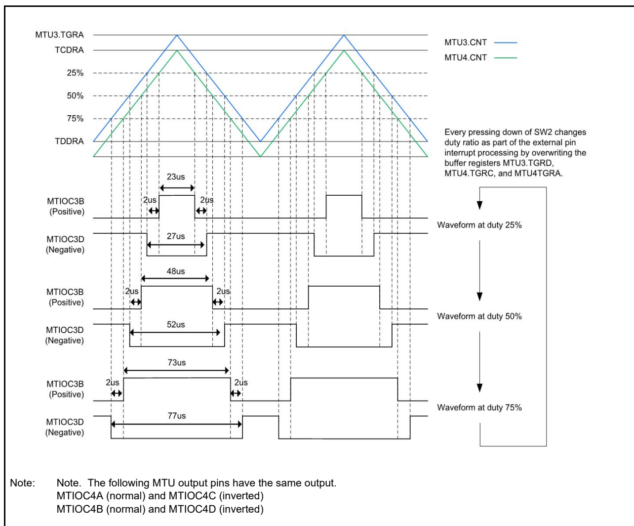
Figure 6.1 Timing Diagram
