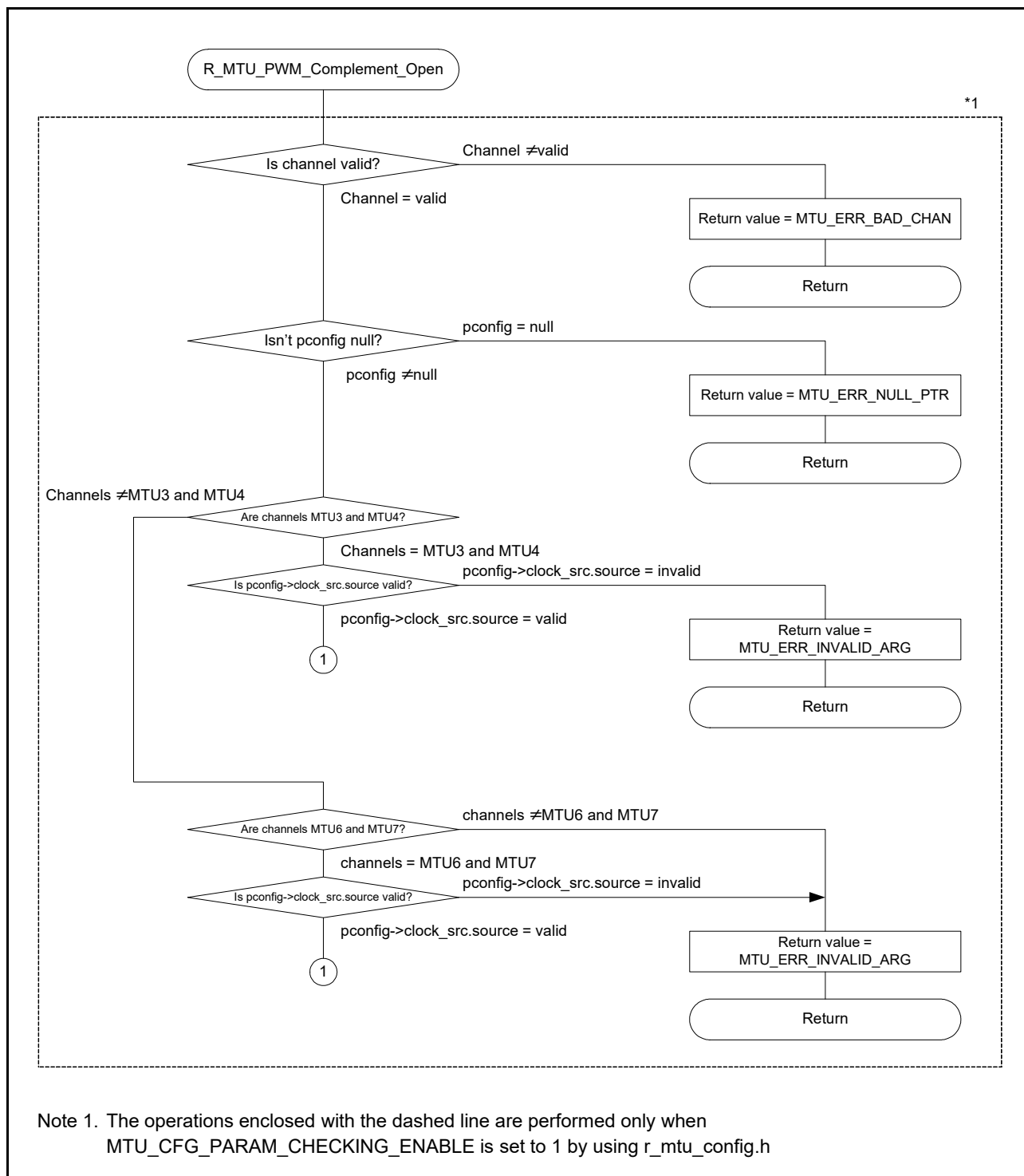
Figure 6.17 Complementary PWM Mode Setting (1)
