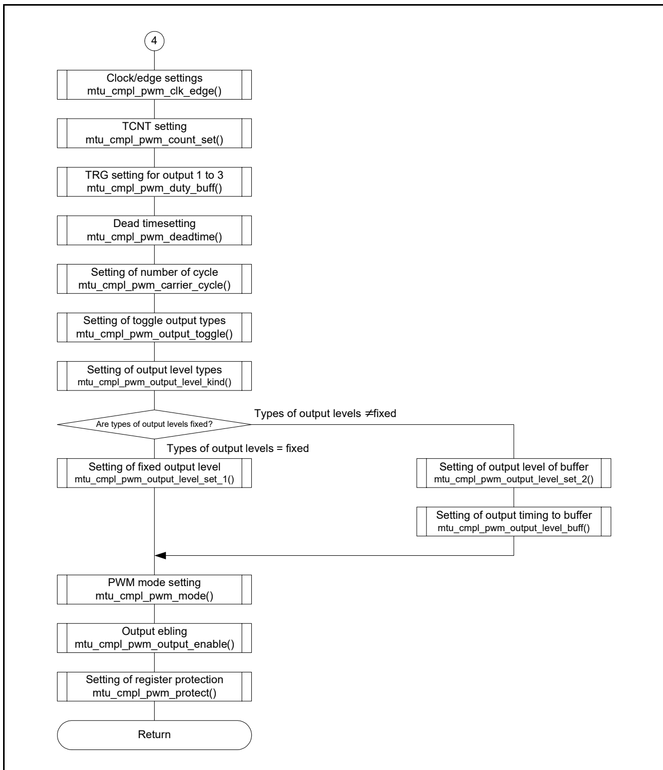
Figure 6.21 Complementary PWM Mode End Processing (5)
