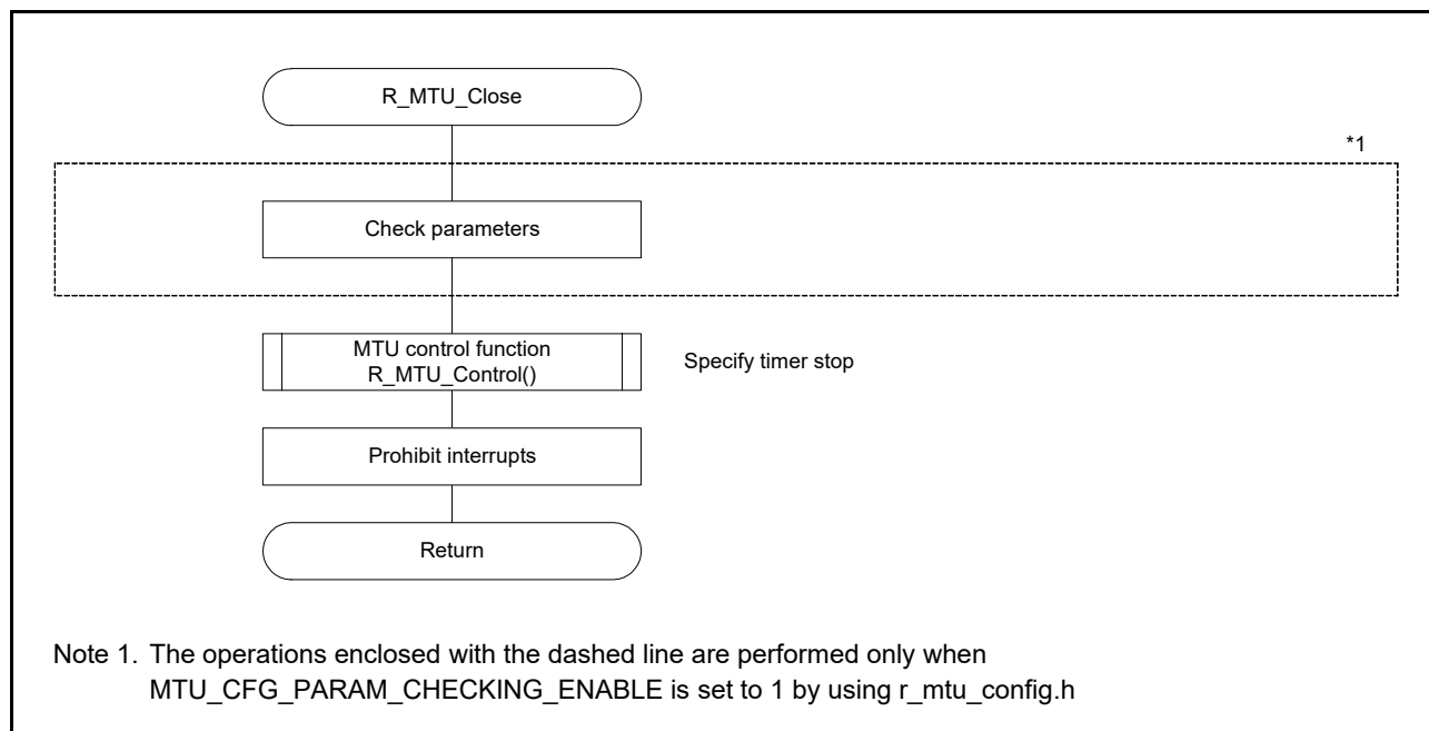
Figure 6.29 MTU End Processing
