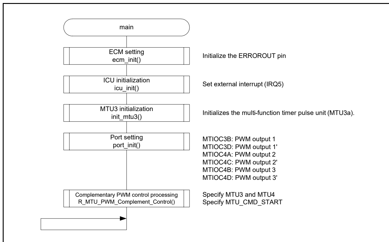
Figure 6.15 Main Processing
