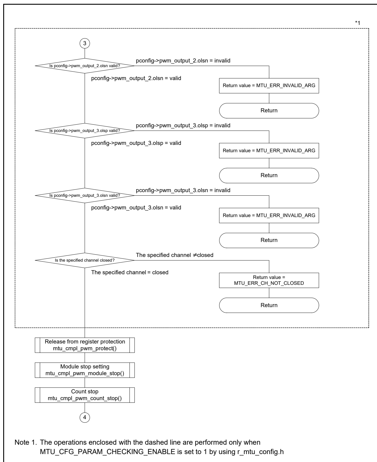
Figure 6.20 Complementary PWM Mode End Processing (4)
